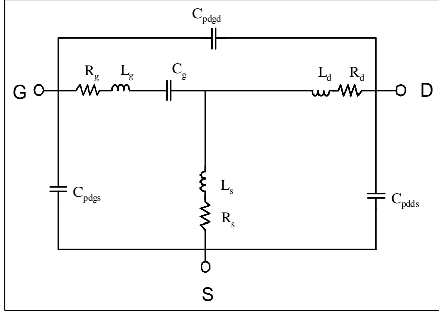
Figure 4. High frequency model of the forward-biased device.
