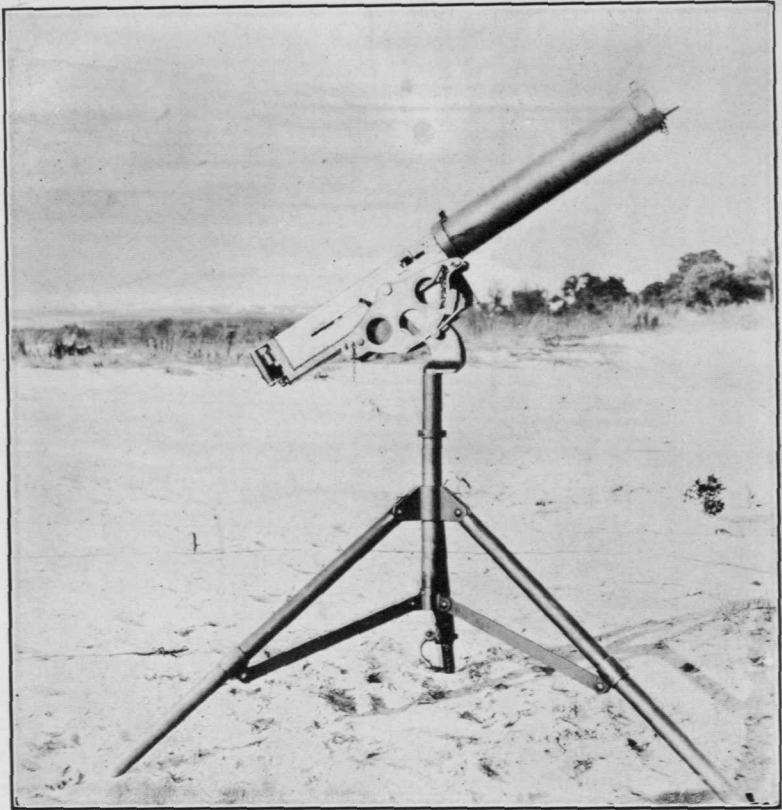
FIG. 3. .50 CALIBER MACHINE GUN, MODEL 1921. (WATER COOLED)
