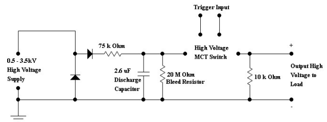
Fig. 1. Experimental Setup.
