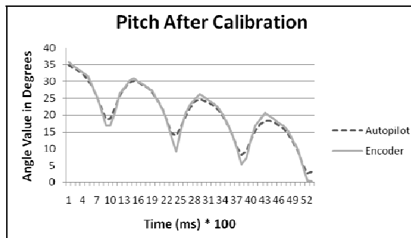
Figure 2. After calibration.
