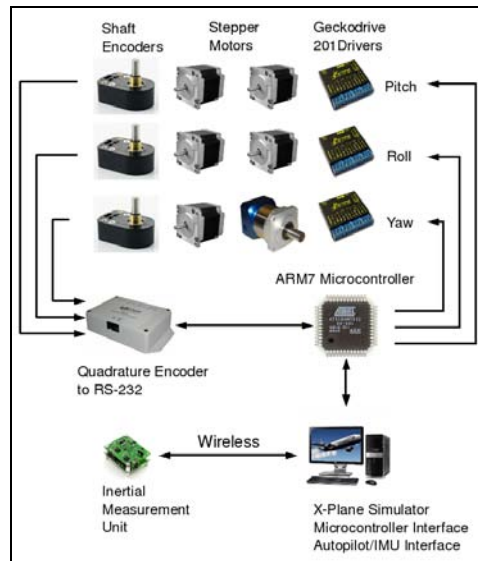
Figure 7. System diagram.
