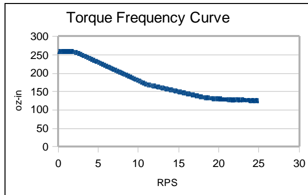
Figure 6. Stepper torque vs. frequency.
