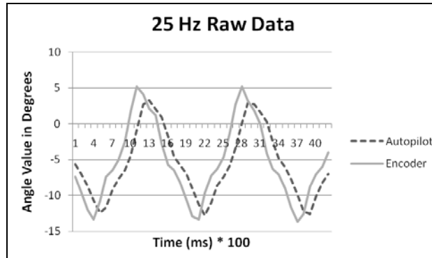
Figure 3. Before shifting.
