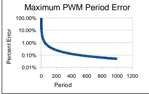
Figure 8. Maximum error curve for the PWM period values.
