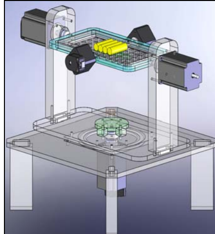
Figure 5. Three-axis gimbaled platform.
