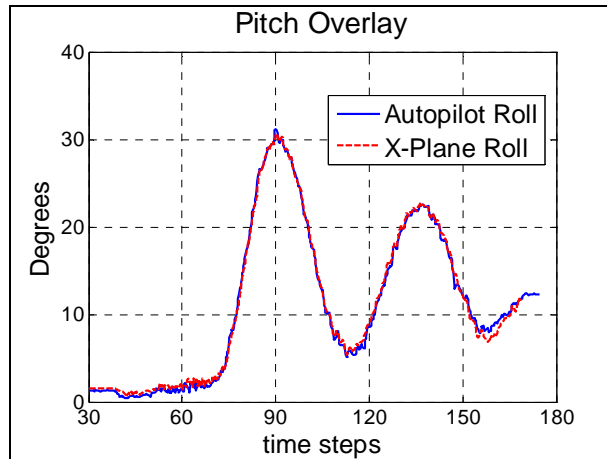
Figure 9. Pitch overlay.
