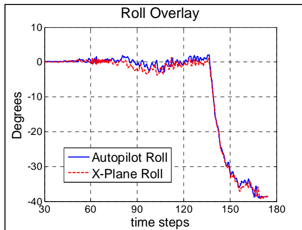
Figure 10. Roll overlay.
