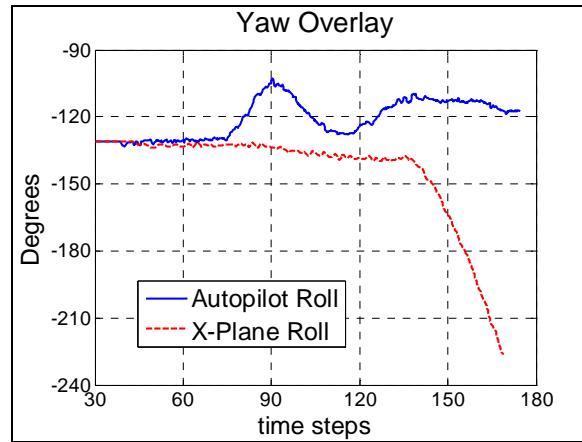
Figure 11. Yaw overlay.
