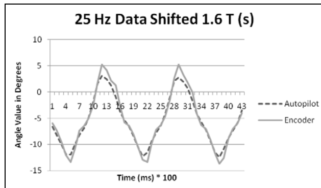
Figure 4. After shifting.
