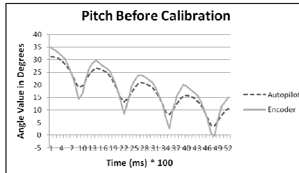
Figure 1. Before calibration.
