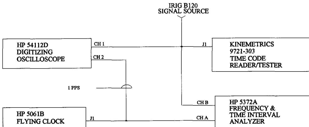
Figure 2. Test Configuration.
