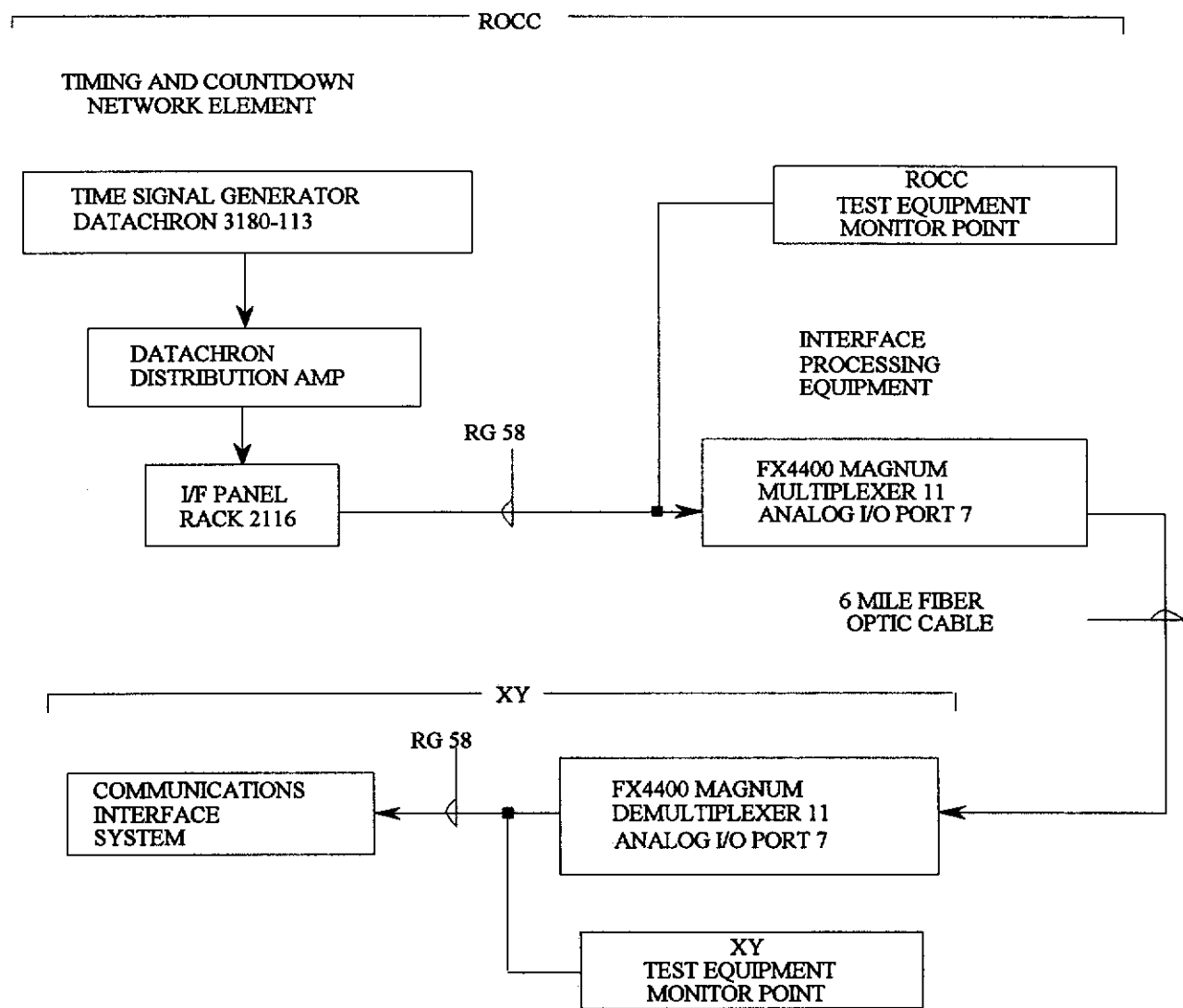
Figure 1. System Configuration.
