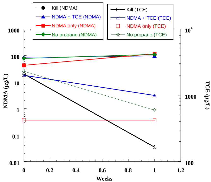
Figure 67. Biodegradation of NDMA and TCE by indigenous bacteria in aquifer samples from Air Force Plant PJKS, CO. All microcosms except the controls were pre-incubated with propane for 2 weeks prior to addition of NDMA or NDMA/TCE to stimulate propane-oxidizing bacteria.
