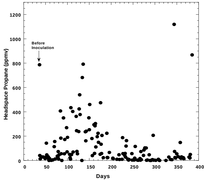
Figure 48. Headspace propane concentrations in the laboratory MBR. The headspace propane levels are provided in ppmv. The reactor was inoculated on Day 37.
