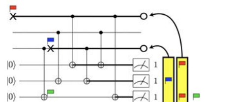
Figure 4.6: Message passing: flags raised by the first level of error correction are tracked through the circuits of the second level of error correction to aid in the diagnosis of level-1 errors. In this example, the blue and red flags match the measured syndrome and are thus identified as being the most likely errors.
