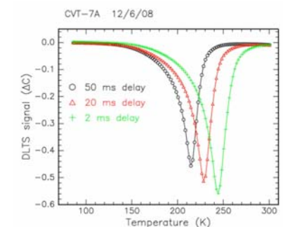
Figure 6.7: The raw DLTS signal versus temperature for nominally 5 nm thick thermal oxides without a post-metallization anneal.
