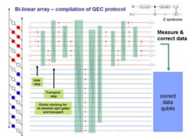
Figure 4.3: Compilation of the DiVincenzo-Aliferis QEC protocol (Z-symptom shown) for the Steane code on the bi-linear array showing gate and transport schedules. Compounding such protocols for X and Z syndrome extraction into the extended rectangle for encoded gates (e.g. CNOT) and subsequent concatenation allows for the determination of a lower bound of the fault-tolerant thresholds (pseudo and asymptotic).
