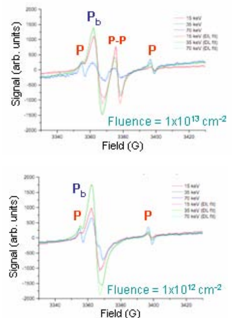
Figure 5.5. ESR spectra and fits for the samples with ~5 nm thermal oxide: a) implanted with 1 \times 10^{13} \text{ cm}^{-2} fluence and energies of 15, 35 and 70 keV, b) implanted with 1 \times 10^{12} \text{ cm}^{-2} fluence and the same energies.
