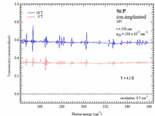
Figure 5.4. Spectrum of an ion-implanted sample of Si(P) in both zero magnetic field (bottom, dashed, red line) and in magnetic field of 18T (top, full, blue line).
