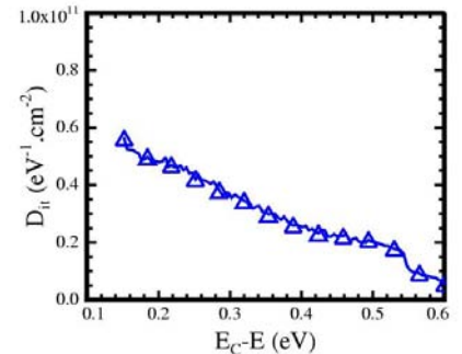
Figure 6.2: DLTS measurements of interface trap densities for a 5 nm oxide implanted with 15 keV P to a fluence of 1 \times 10^{11} \text{ P/cm}^2 and then rapid thermally annealed at 1100°C, 5s prior to capacitor formation.
