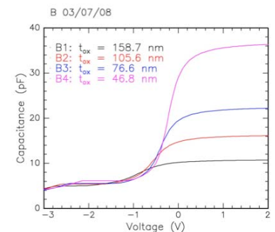
Figure 6.5: Capacitance-Voltage curves for the field oxide having undergone a post-oxidation anneal and various etches to thicknesses indicated in the figure.
