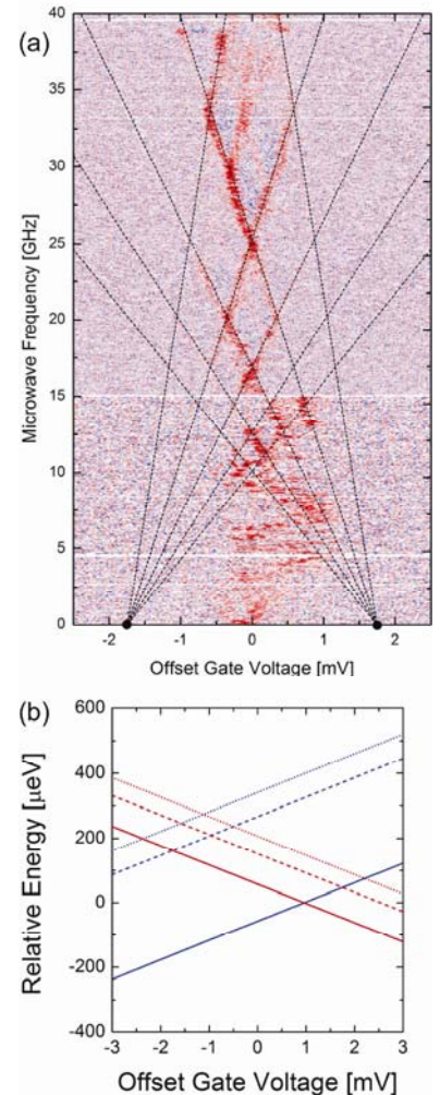
Figure 3.8: 4-P-Atom device. (a) SET signal as a function of applied gate voltage and applied microwave frequency. Dotted lines are a fit to theory. (b) Energy levels of the (P_3-P)^{2+} system.
