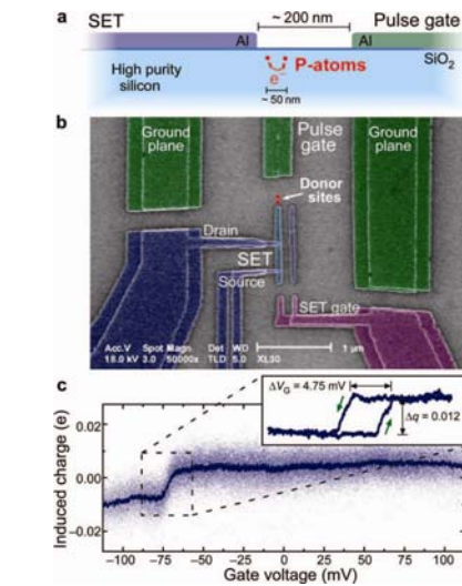
Figure 3.7: (a) Schematic and (b) colour-enhanced SEM image of 2-P-Atom device. (c) Induced charge on SET island, measured at MHz bandwidth for several gate sweeps with averaged data in solid. Inset of averaged charge transfer shows hysteresis in gate voltage.
