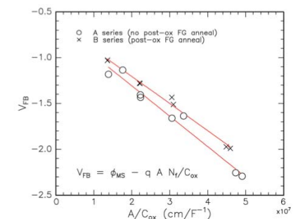
Figure 6.6: Flat band voltage determined from the C-V curves as a function of the A/C_{ox} for the etched back field oxides.
