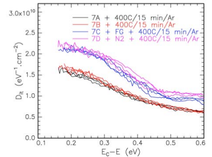
Figure 6.9: Interface trap densities, D_{it} , versus tap energy relative to the conduction band edge obtained from DLTS measurements on 5 nm oxides after various post-metallization anneals
