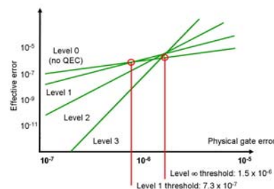
Figure 4.4: Error thresholds (lower bounds) for the encoded CNOT gate at various levels of concatenation, showing pseudo-thresholds (Level 1 = 7.3 \times 10^{-7} ) and asymptotic threshold estimate (Level \infty = 1.5 \times 10^{-6} ) for a conservative set of inputs with respect to physical times and error rates for gates, transport and measurement.
