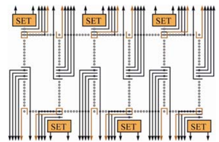
Figure 4.1: Bi-linear Si:P array with horizontal and vertical transport rails into and out of central interaction regions.
