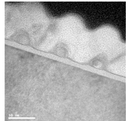
Figure 6.12: Transmission electron microscopy image of a cross-section through the three aluminium gate fingers showing details of the aluminium oxide interfacial regions surrounding each finger which provide electrical isolation between the various levels of metallisation.
