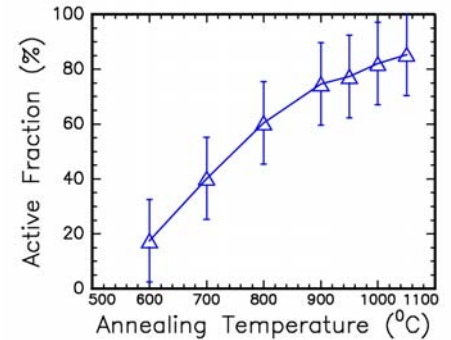
Figure 6.1: Activation fraction of P donors versus annealing temperature for 5s anneals of P, 15 keV, 1 \times 10^{13} \text{ cm}^{-2} implants into high-resistivity B-doped substrates capped with a 5nm thermally-grown oxide. 5nm thermally grown oxide.
