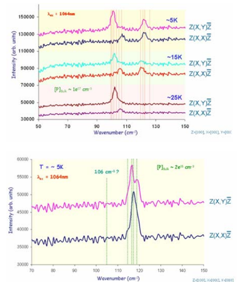
Figure 5.11. Polarised NIR micro-Raman measurements of bulk doped Si:P at low temperatures.
