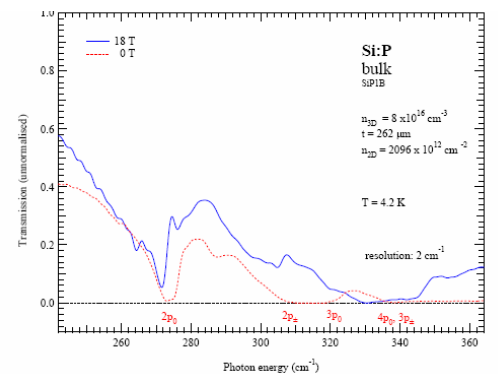
Figure 5.1. Spectrum of a “lightly” doped sample of \text{Si(P)} in both zero magnetic field (bottom, dashed, red line) and in magnetic field of 18 T (top, full, blue line).
