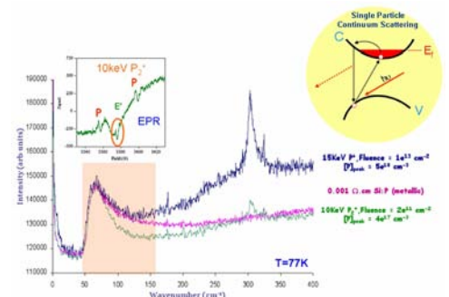
Figure 5.12. Single particle scattering from bulk doped (metallic) and ion implanted Si:P. The inset ESR spectrum is also from the 10\text{keV} molecular P implant.
