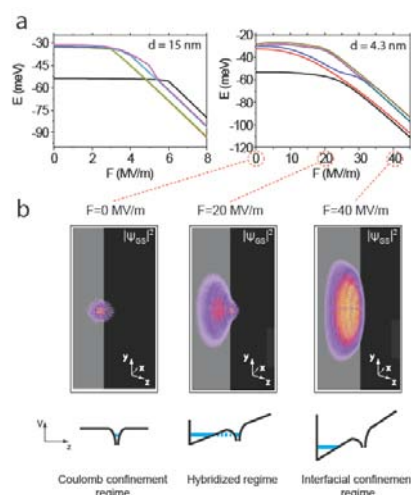
Figure 4.5: a) Stark shift of donor orbital levels as a function of field strength and donor depth. b) Hybridization of donor states near an interface: NEMO calculations used to interpret experimental data.
