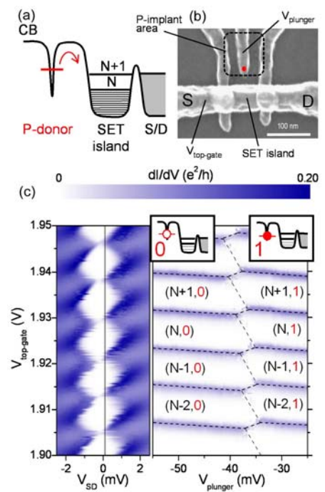
Figure 3.12: (a) Energy landscape and (b) SEM image of locally doped Si:P MOS device with SET island acting as induced electron reservoir. (c) Voltage spectroscopy of the device reveals individual single electron transfers from P-atom to SET island.
