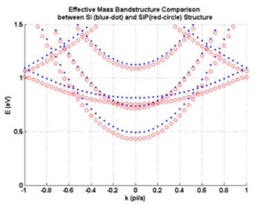
Figure 4.7: Dispersion of a 2 \times 2 \text{ nm}^2 nanowire with and without centrally embedded line of P atoms. A 60meV downshift due to the insertion of the P impurities can be observed.
