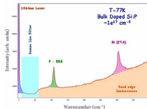
Figure 5.9. Spectroscopy of bulk doped Si:P ( \sim 1 \times 10^{17} \text{cm}^{-3} ) when using 1064nm (NIR) laser excitation. Spectral features have been coloured for identification and include: a Rayleigh scattered laser peak at 0\text{cm}^{-1} , the spectral profile of the Raman Notch (line) filter, silicon band edge luminescence, a second order silicon acoustic phonon (2TA) and the phosphorus donor 1S(A_1) to 1S(E) electronic transition (i.e. absorption) at \sim 106\text{cm}^{-1} .
