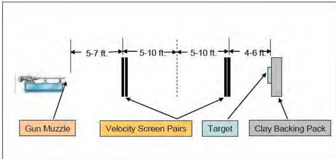
Figure 4. Typical Indoor Range Setup
