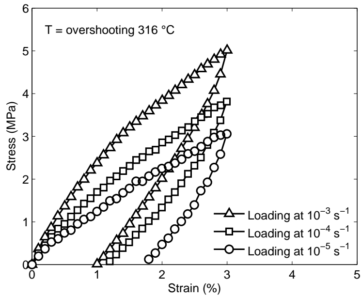
Figure 9.2: Overshooting the Test Temperature of 316\text{ }^{\circ}\text{C} . The results of the Monotonic Loading and Unloading are exhibited.
