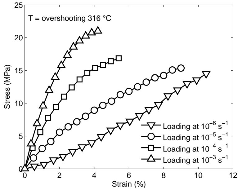
Figure 9.1: Overshooting the Test Temperature of 316\text{ }^{\circ}\text{C} . The results of the Tension to Failure Tests in Monotonic Loading are exhibited.
