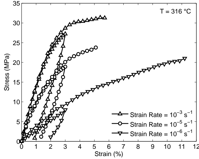
Figure 6.2: Stress-Strain Curves Obtained for PMR-15 in Loading/Unloading Tests Constant Strain Rates of 10^{-3} , 10^{-5} , and 10^{-6} \text{ s}^{-1} at 316^\circ\text{C} Compared to Tension to Failure Results. The Dependence of the Unloading Behavior on the Strain Rate is Evident.
