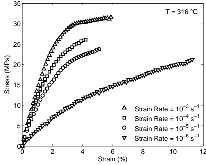
Figure 6.1: Stress-Strain Curves Obtained for PMR-15 in Tensile Test to Failure Conducted at Constant Strain Rates of 10^{-3} , 10^{-4} , 10^{-5} , and 10^{-6} \text{ s}^{-1} at 316^\circ\text{C} . The Dependence of the Stress-Strain Behavior on the Strain Rate is Evident.
