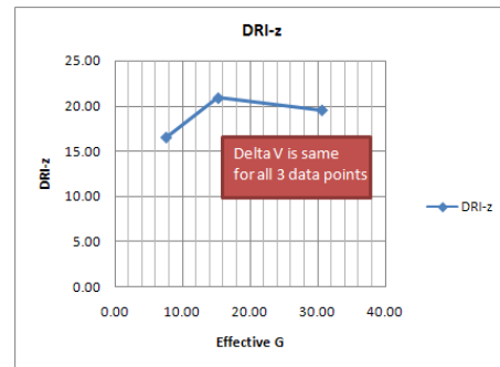
Figure 15: DRI-z Response
