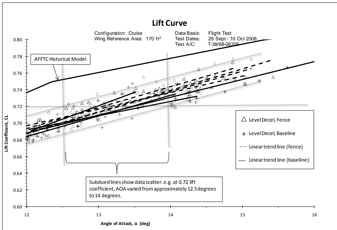
Figure 130. Expanded Baseline versus Modified Aircraft Lift Curve
