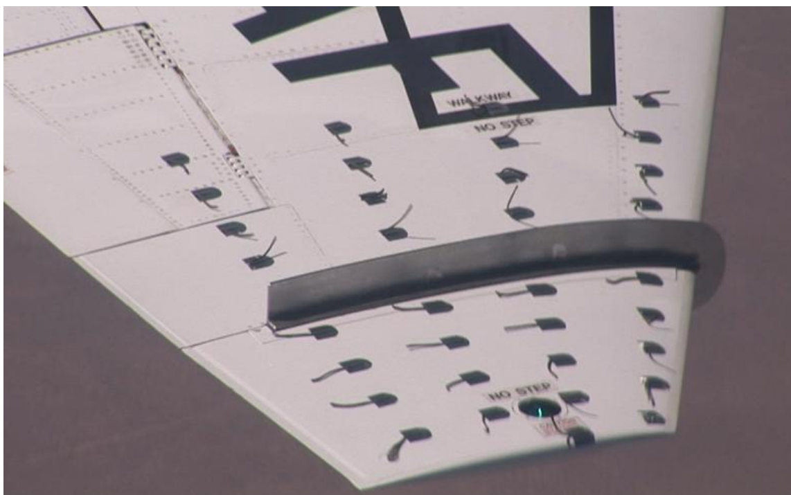
Figure 202. Fence Tufted Wing at 14.2^\circ AOA (0.94 normalized) and 146 KCAS
