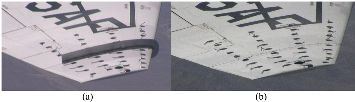
Figure 138. Fence and Clean Tufted Wings at 8.4 degrees AOA (0.56 normalized) (a) 185 KCAS (b) 188 KCAS
