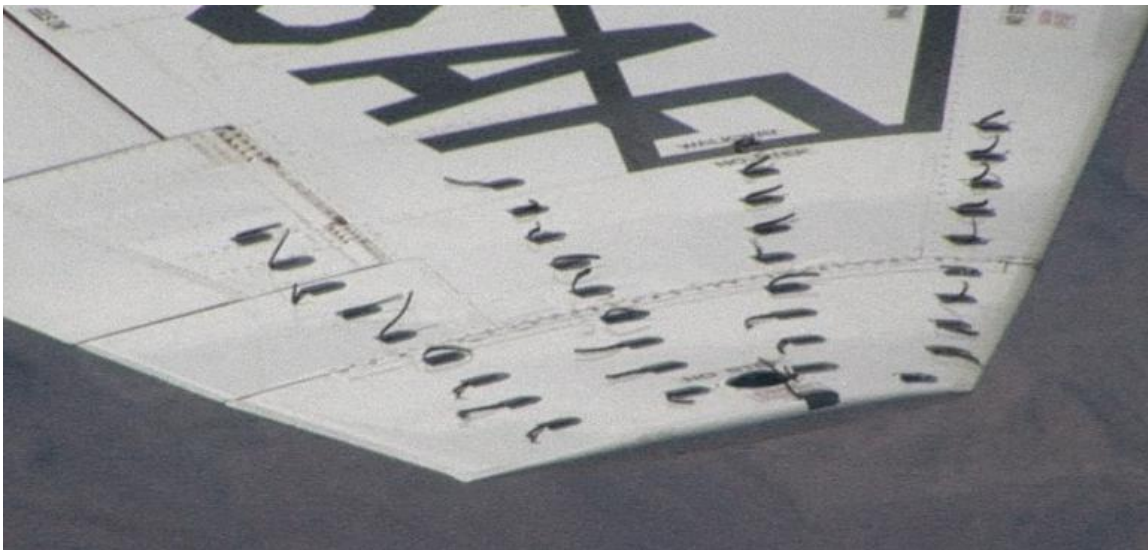
Figure 177. Clean Tufted Wing at 8.6^\circ AOA (0.58 normalized) and 183 KCAS
