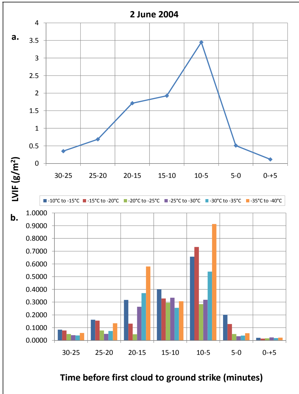
Figure 8. a. Total LVIF for 2 June 2004. b. LVIF of each thermal layer for 2 June 2004.
