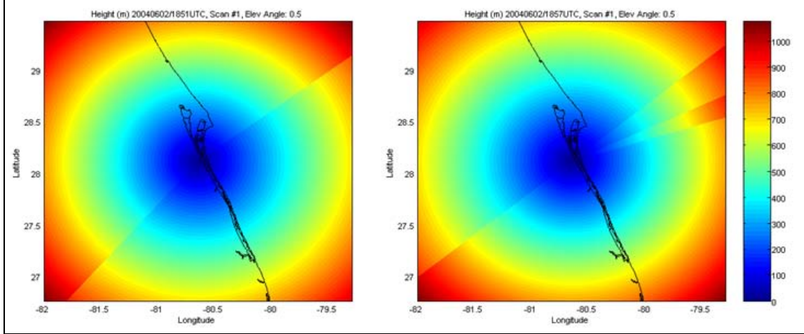
Figure 4. Discrepancies with height between two scans at the same elevation angle (0.5°).
