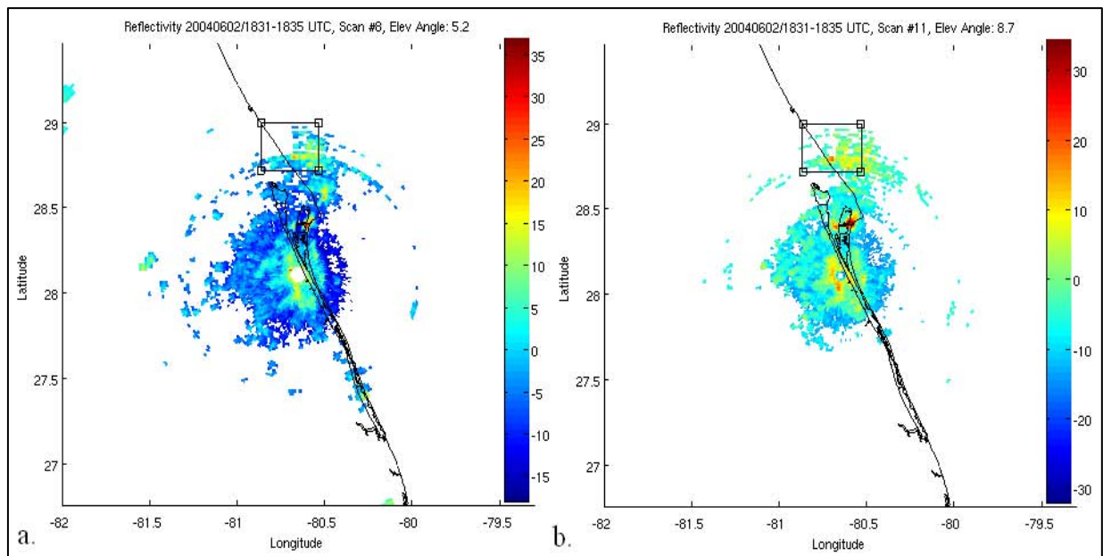
Figure 6. Example from 2 June 2004: a. Elevation Angle 5.2°; b. Elevation Angle 8.7°.
