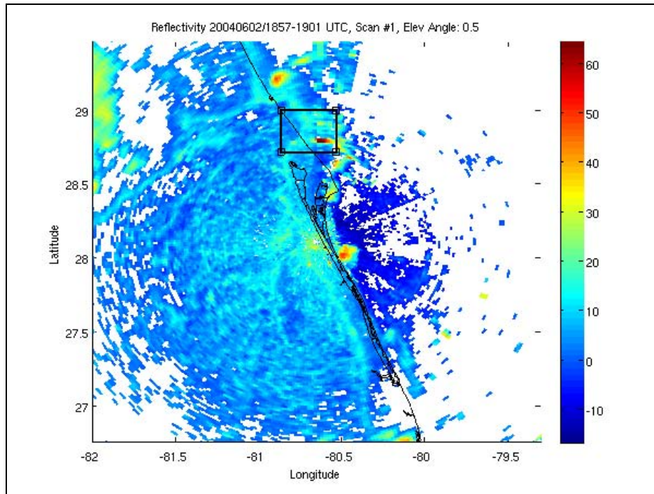
Figure 3. Sample of the reflectivity grid taken from 2 June 2004, elevation angle 0.5^\circ . The boxed area indicates the storm location.
