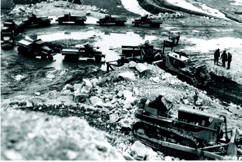
(Above) 1903rd EAB engineers haul rock from surrounding hills to be crushed for use in airfield and road construction. The greatest single day haul for the 1903rd as of March 1952 was 855 truckloads.
