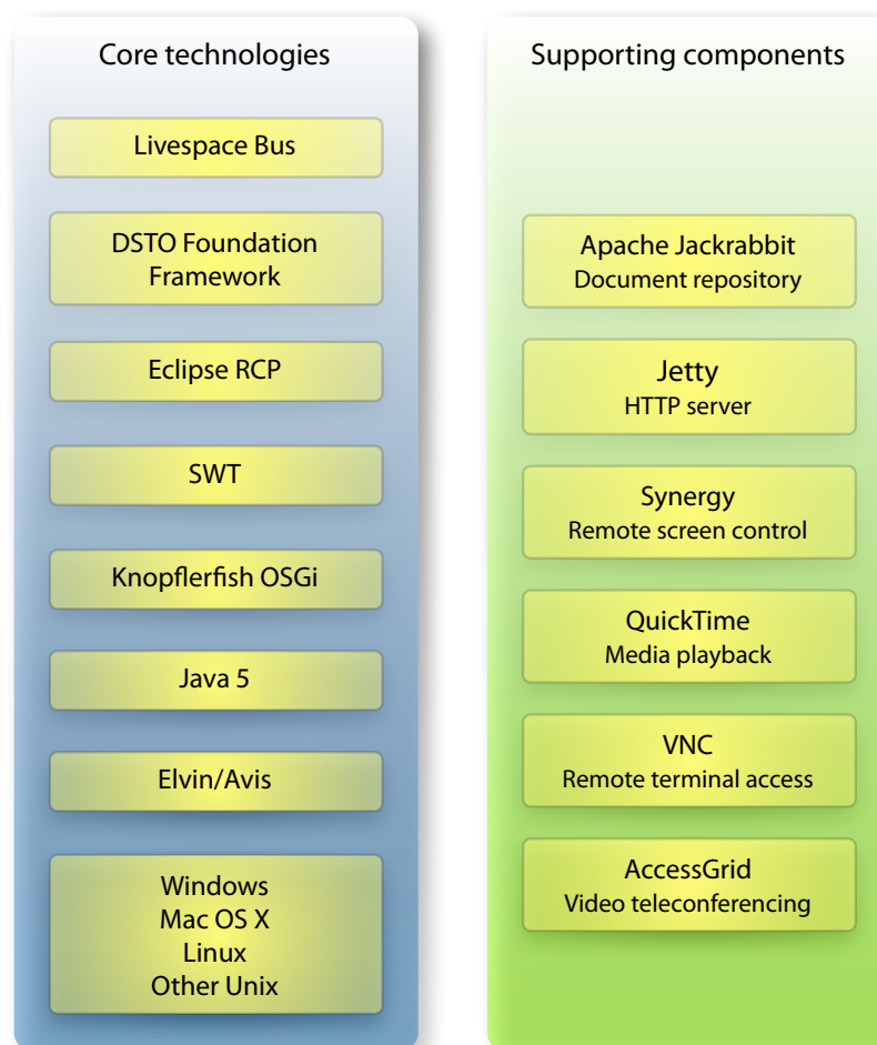
Figure 32. Technology foundations for Livespaces
