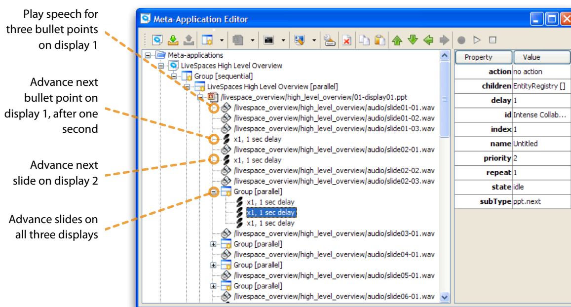
Figure 28. The internal structure of a meta application
