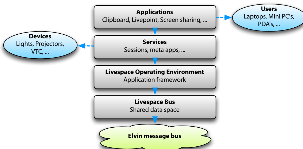
Figure 2. The Livespace architecture stack
