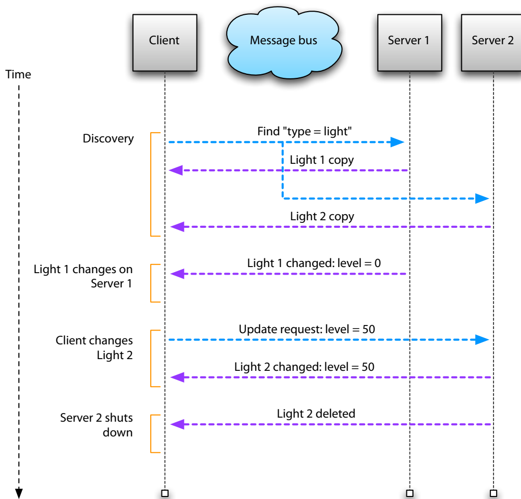
Figure 6. Entity replication sequence
