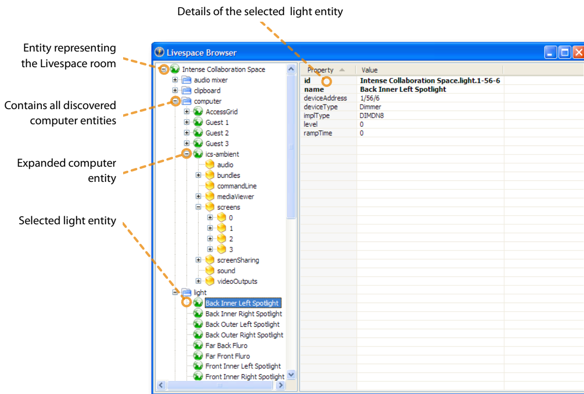
Figure 5. The Livespace Browser application
