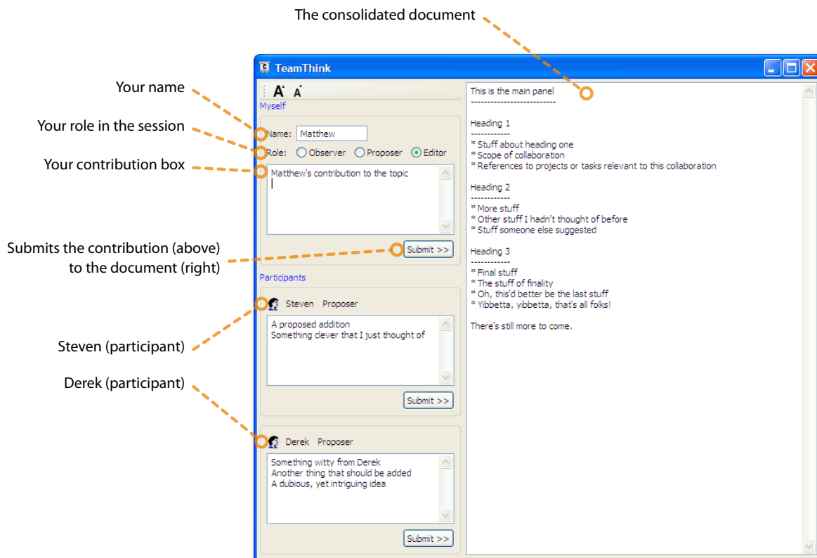
Figure 12. The TeamThink window
