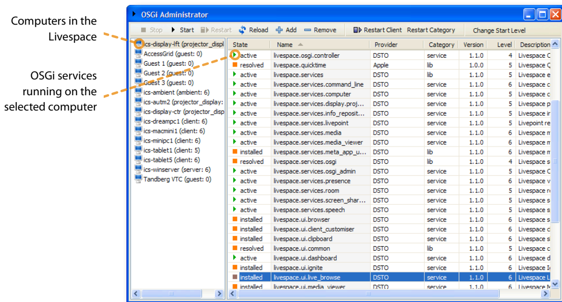
Figure 29. The OSGi service administration window
