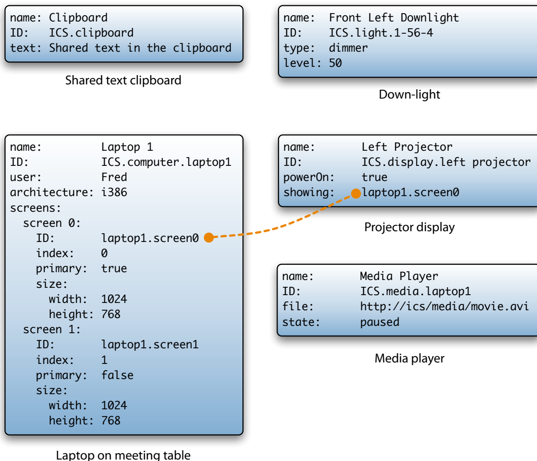
Figure 3. Some example Livespace entities
