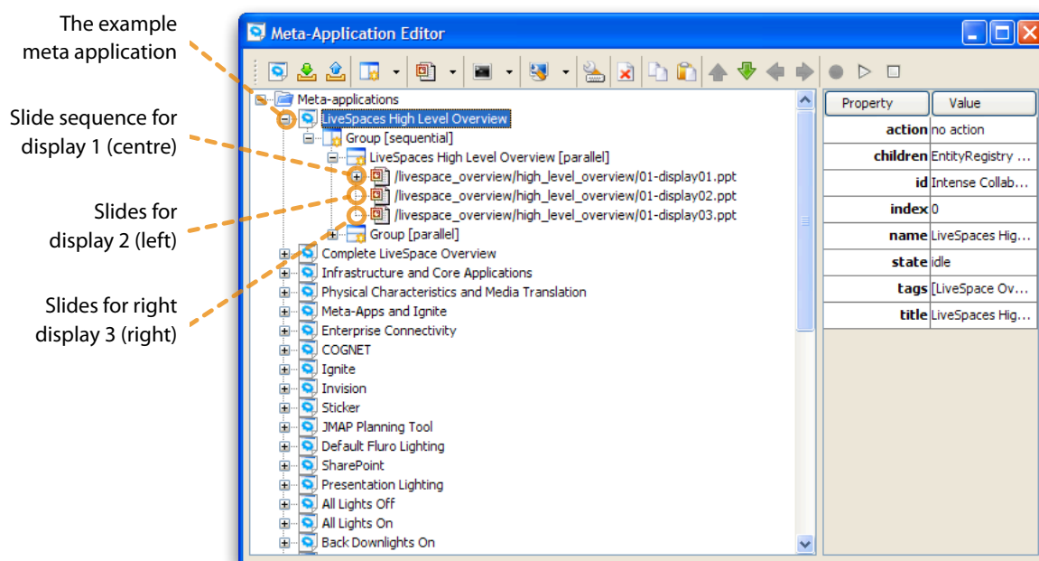
Figure 26. The Meta Application Editor
