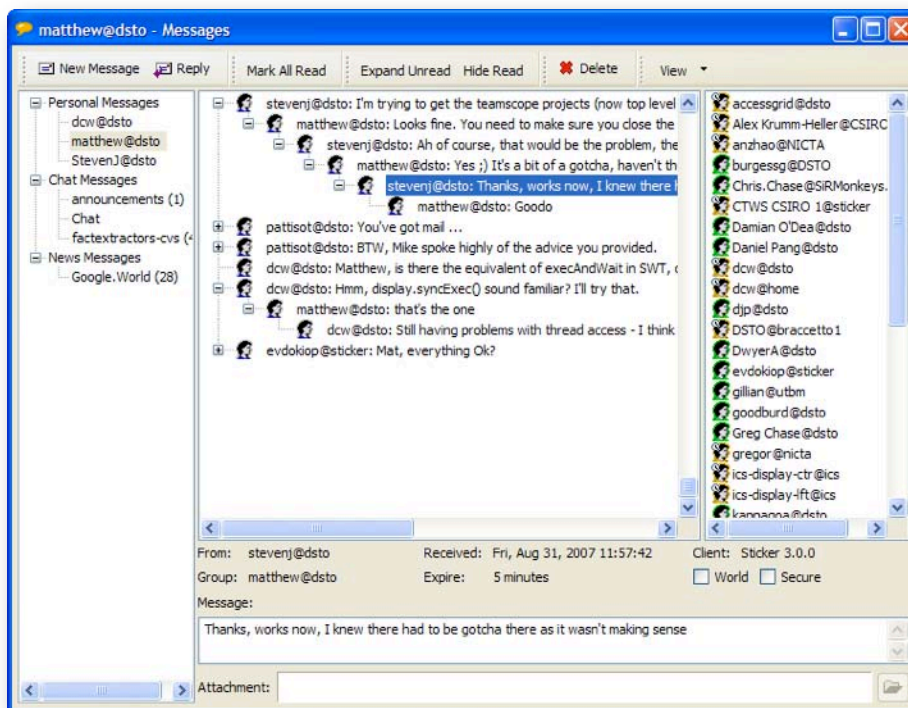
Figure 23. The Sticker Messages window
