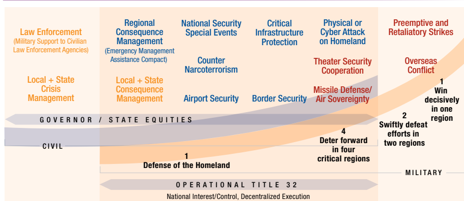
Figure 2. Governor/State Equities
