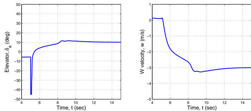
Figure 4.3: Nonlinear W-velocity controller response to a -3 \text{ m/s} step input in w velocity for the YAK-54 with a 10% overshoot.
