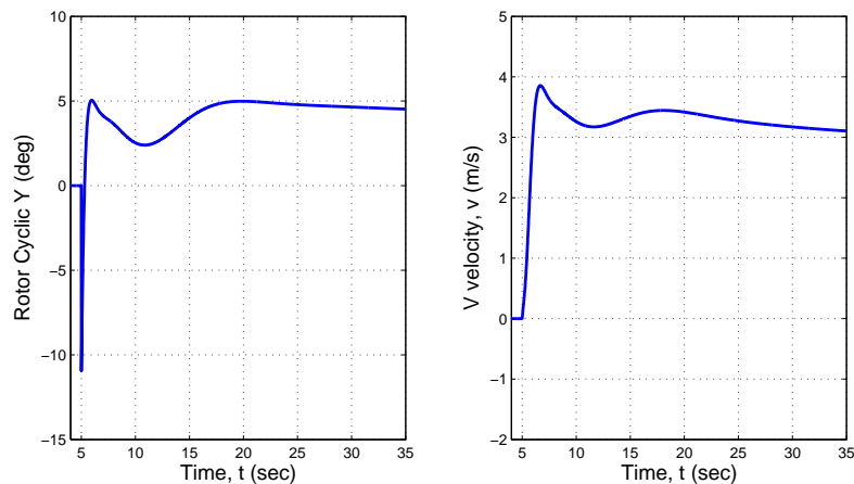
Figure 4.10: Linear V-velocity controller response for the Flexrotor to a 3 \text{ m/s} step input in v velocity with a 21% overshoot.
