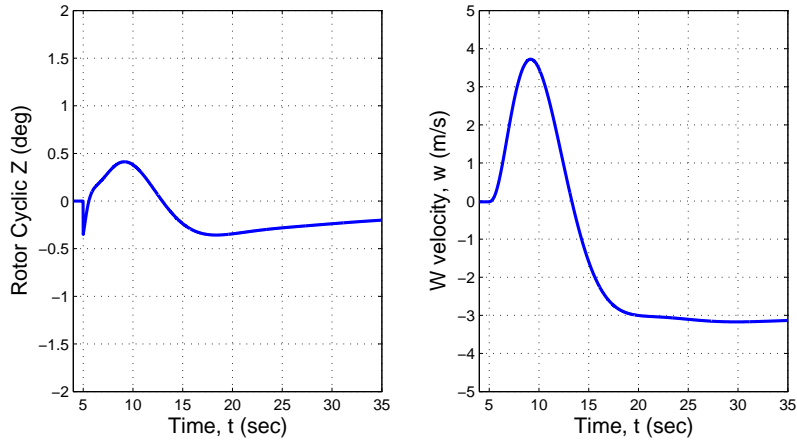
Figure 4.9: Linear W-velocity controller response for the Flexrotor to a -3 \text{ m/s} step input in w velocity.
