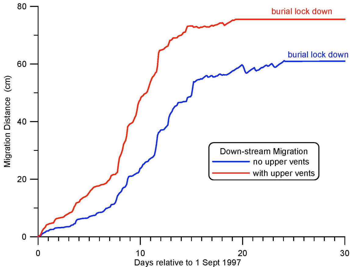
Figure 4: Simulated down-stream migration history of dead weight anchor based on proxy hydrograph from Missouri River at Omaha, NE (USGS gage station #06610000). Dry bulk mass = 15.88 kg (dry weight = 35 lb)
