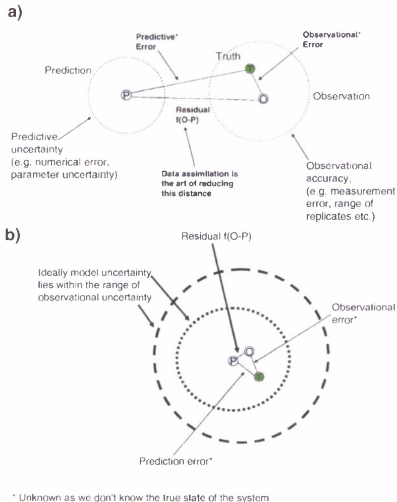
Fig. 1. Schematic diagram of the relationships between model prediction (P), observations (O) and the true state of the system (T). Both P and O are assumed to have a halo of uncertainty. a) shows the case for a model with no skill and b) shows the case for the ideal model, with inner circle representing model uncertainty and outer circle representing observational uncertainty.
