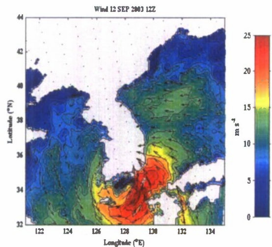
Figure 1: COAMPS wind ( \text{m s}^{-1} ) and wind vector output for 12 UTC SEP 12 indicating landfall of Typhoon Maemi near Masan, South Korea.
