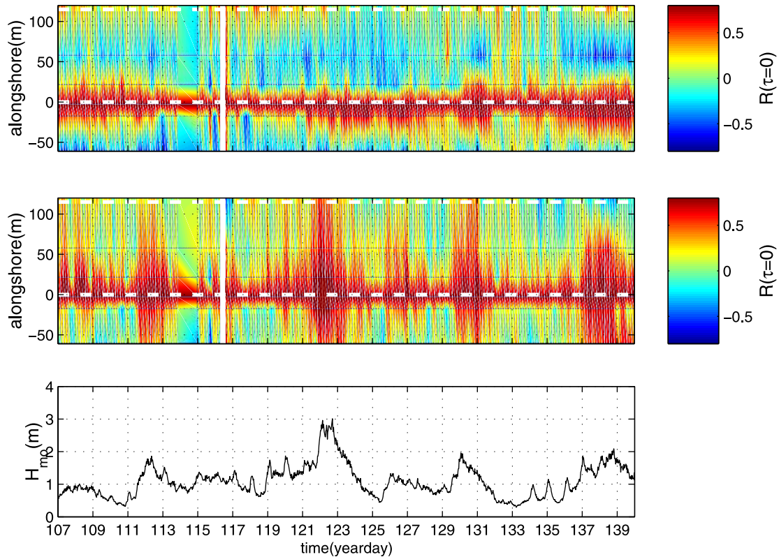
Figure 10. Cross correlations of (top) u_{\text{VLF}} and (middle) v_{\text{VLF}} with respect to measurements at PUV6 located within the rip channel at y = 0 in the alongshore array at zero time lag. Dashed line represents location of the rip channels. (bottom) H_{m0} given for reference.
