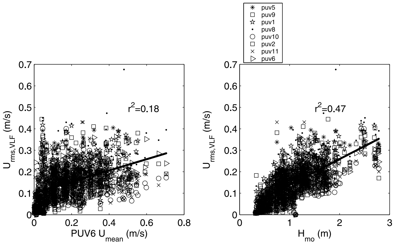
Figure 9. U_{rms,VLF} plotted versus (left) U_{mean} measured at PUV6 and (right) H_{mo} .
