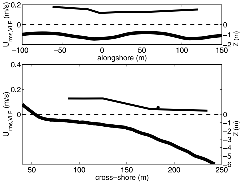
Figure 8. U_{rms,VLF} averaged over year days 111–120 (top) within the alongshore array and (bottom) in the cross shore. The 95% confidence interval is represented by the thickness of the U_{rms,VLF} curve. The depth profiles are shown as a thick curve (depth labeled on the right-hand side). U_{rms,VLF} measured at by the ADCP in the neighboring rip channel is represented by black circle. The dashed line represents zero intensity and mean sea level.
