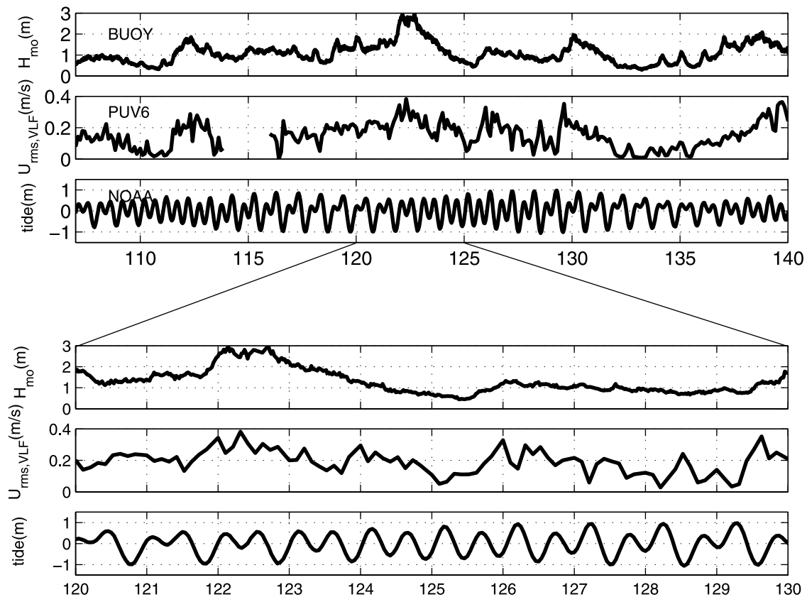
Figure 7. Significant wave height measured at the wave buoy for reference is shown in the first panel. Variance of U_{VLF,rms} for PUV6 located within the rip channel is shown in the second panel. Tidal elevation measured at the NOAA station for reference is shown in the third panel. The top three plots span the time period for year days 107–140, while the bottom three plots are expanded views of year days 120–130 to examine the tidal variability.
