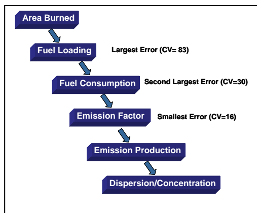
Figure 2. Input variables and errors associated with predicting emissions from wildland fires
