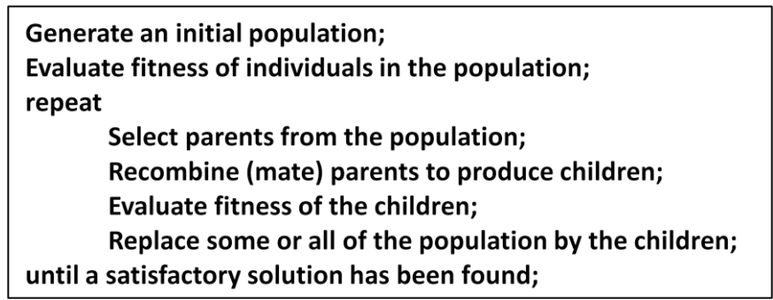
Figure 3. Basic Steps of a Simple GA (20)
