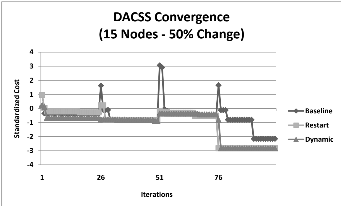
Figure 45. DACSS Convergence - 50% Change (15 Nodes)
