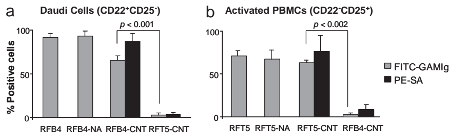
Fig. 4. Binding of mAb-CNTs to target cells. One million cells were incubated with saturating concentrations of RFB4-CNTs or RFT5-CNTs and then incubated either with FITC-GAM1g to detect the mAbs or with PE-SA to detect the B-CNTs and analyzed on a FACScan. (a) The specific binding of RFB4-CNTs to Daudi cells using RFT5-CNTs as a negative control ( P < 0.001 ). (b) The specific binding of RFT5-CNT to activated PBMCs ( >95\% T cells) using RFB4-CNT as a negative control ( P < 0.002 ). Data represent mean \pm SD of at least three independent experiments.
