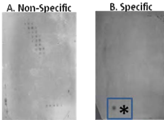
Figure 2. Sample filter hybridizations of CHORI 129 library filters. Filters from CHORI containing the 129 BAC library were hybridized with the fragment of DNA containing Spna1 exon 43. Segment A shows non-specific hybridization signals with a specific hybridization signal shown in B. This signal corresponded to clone CHORI129-99P17 which was used in further experiments.
