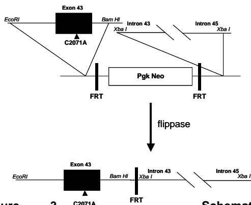
Figure 3. Schematic of mutant vector construction. A diagram of how the design of Spna1 mutant vector C2071A Targeted Allele to construct the Cys to Ala change is shown.
