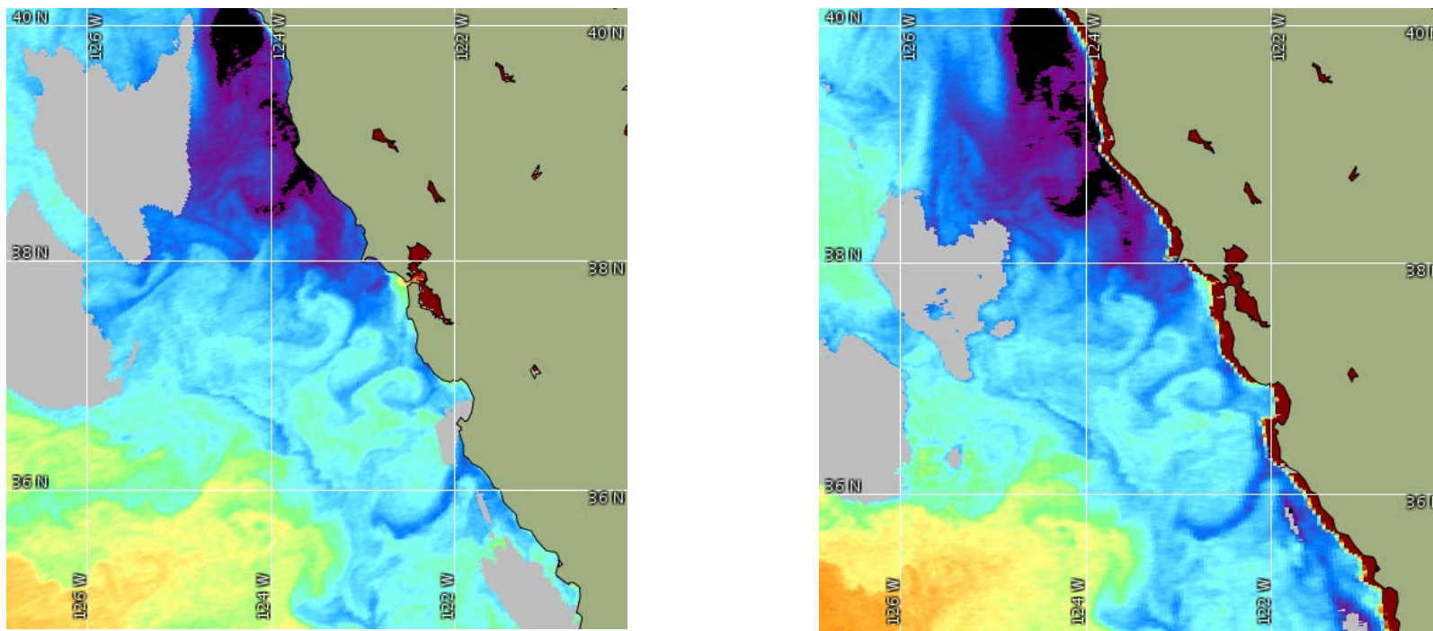
Figure 7. Advanced Very High Resolution Radiometer (AVHRR) satellite imagery of sea surface temperature ( ^{\circ}\text{C} ) of the area of operation during the PaCOOS cruise of June 2008. These images were taken on 24 June 2008 at 2031 UT (left) and 2212 UT (right).
