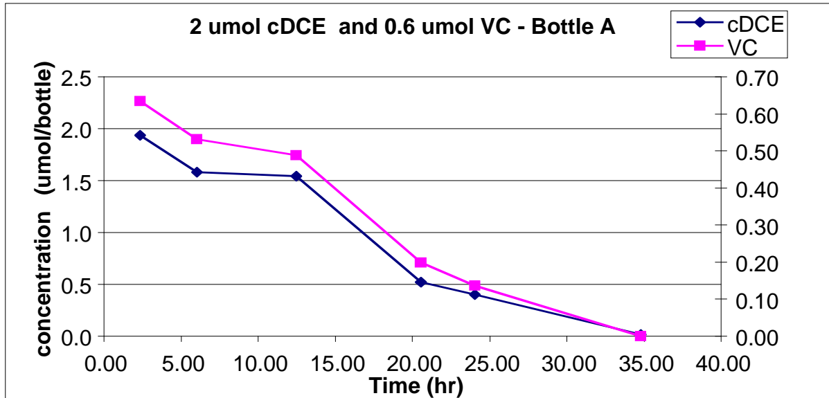
Figure 2.4 Degradation of cDCE and VC at Highest VC Level.
