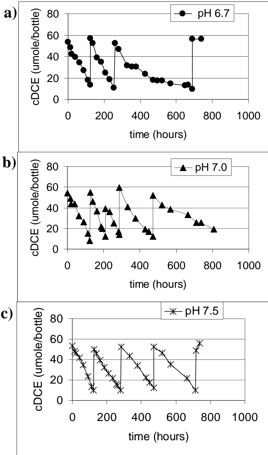
Figure 1.2 Concentration of cDCE Over Time for JS666 Cultures ( OD_{600} = 0.45 ) in MSM with an Initial pH of a) 6.7, b) 7.0, and c) 7.5. cDCE was supplied as the sole carbon source. Single Replicates are Shown for Clarity, but Duplicates Behaved Similarly.
