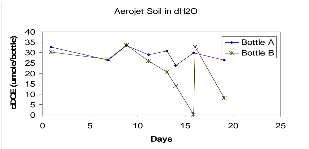
Figure 4.25 Aerojet Soil Inoculated with JS666 Prepared with dH 2 O. Degradation Observed in One Replicate.
