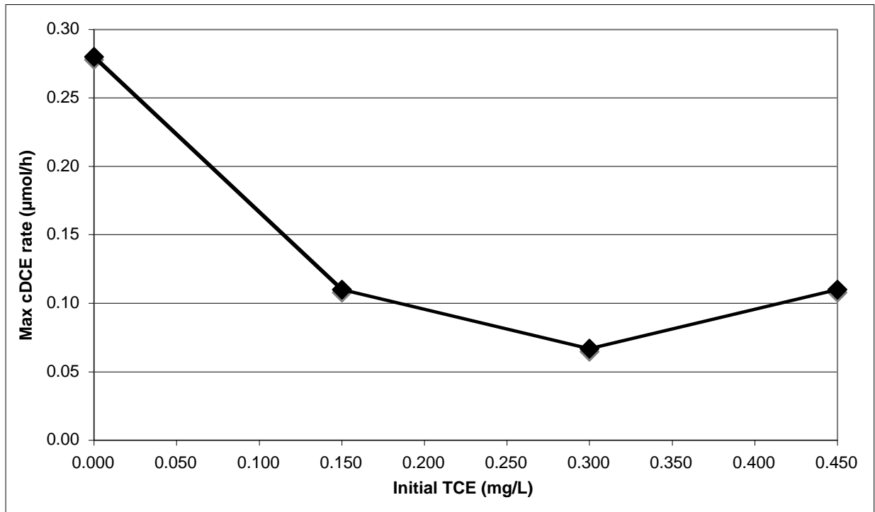
Figure 2.15 Maximum cDCE Degradation Rate as Function of Initial, Aqueous TCE Concentration.
