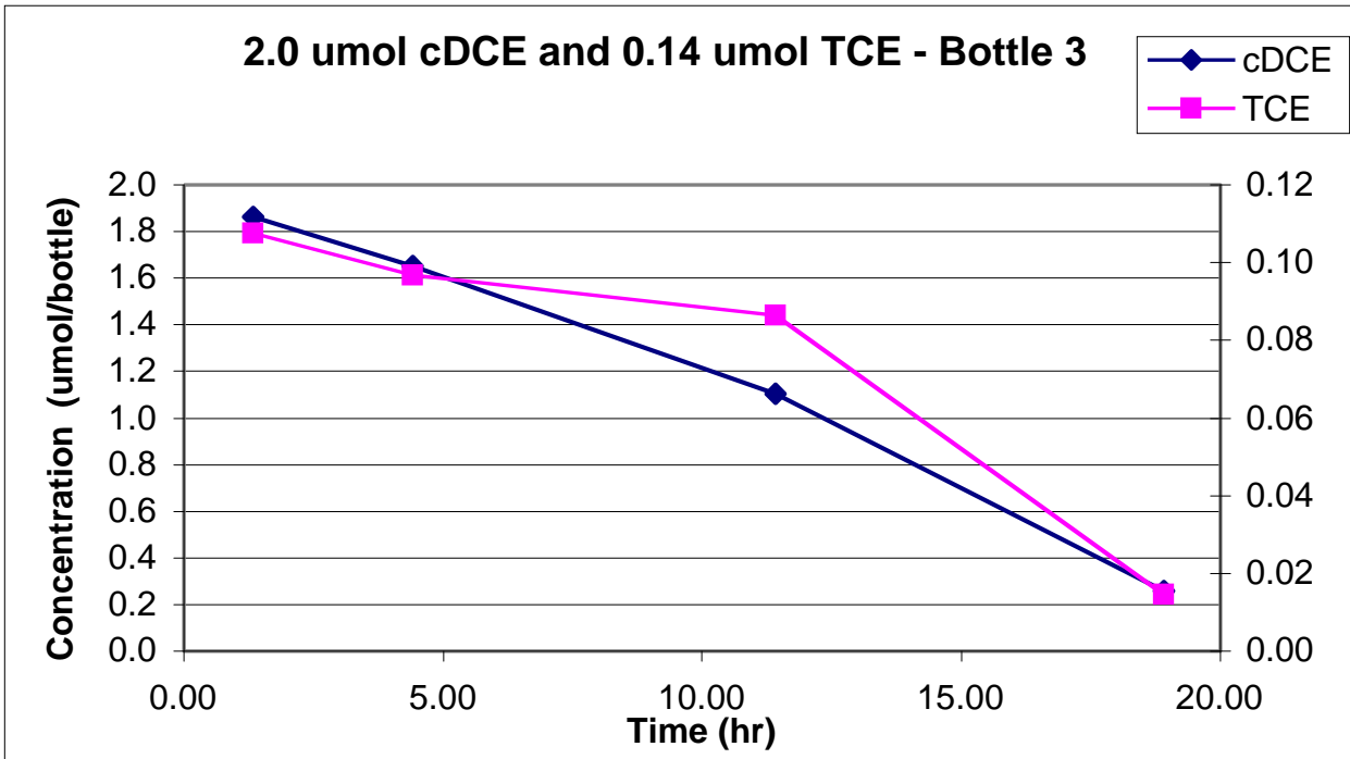
Figure 2.10 Degradation of cDCE and TCE at Lowest TCE Level.
