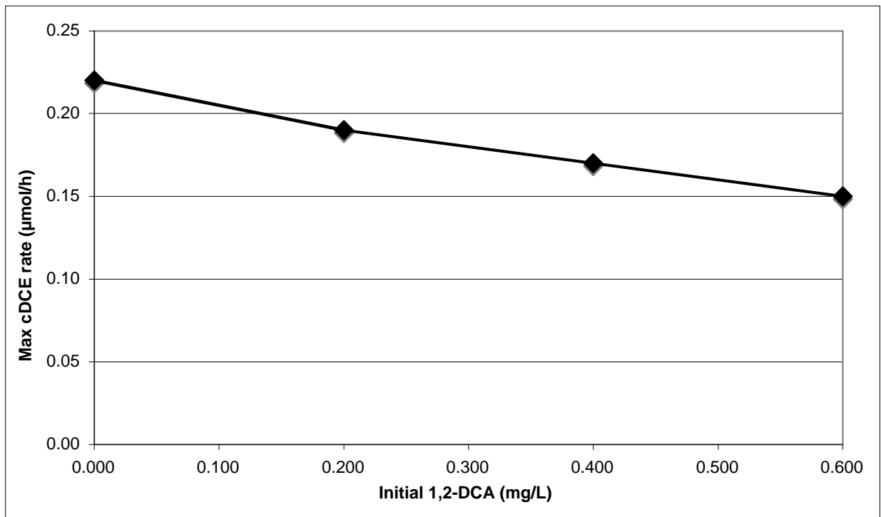
Figure 2.23 Maximum cDCE Degradation Rate as Function of Initial, Aqueous 1,2-DCA Concentration.
