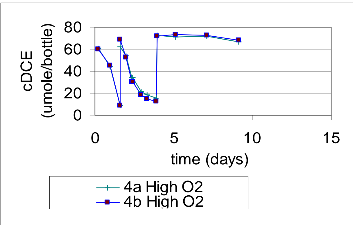
Figure 1.8. cDCE Degradation Patterns in Bottles Challenged with Different Oxygen Levels.
