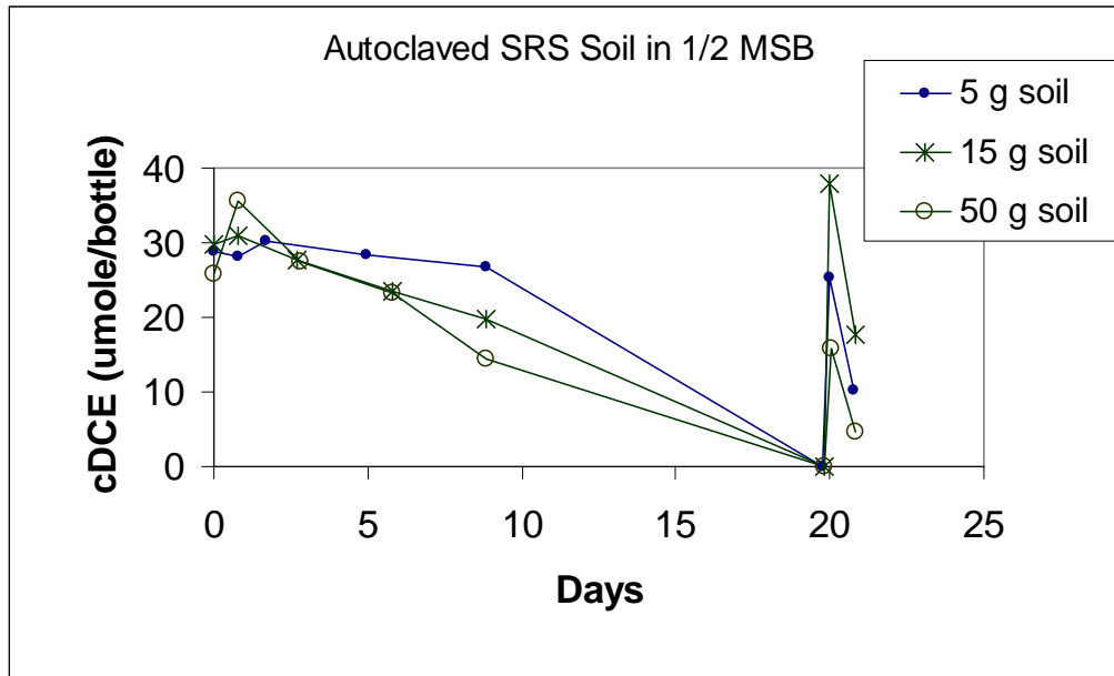
Figure 4.8. Autoclaved SRS Soil Inoculated with JS666 and Amended with 1/2 MSB and 10 mM Ethanol. Results for 5, 15, and 50 grams of soil. Duplicates behaved similarly (not shown).
