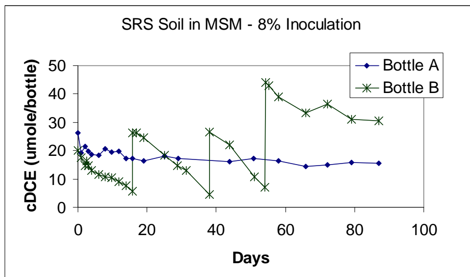
Figure 4.4 SRS Soil in MSM Inoculated With 8% Transfer Culture.
