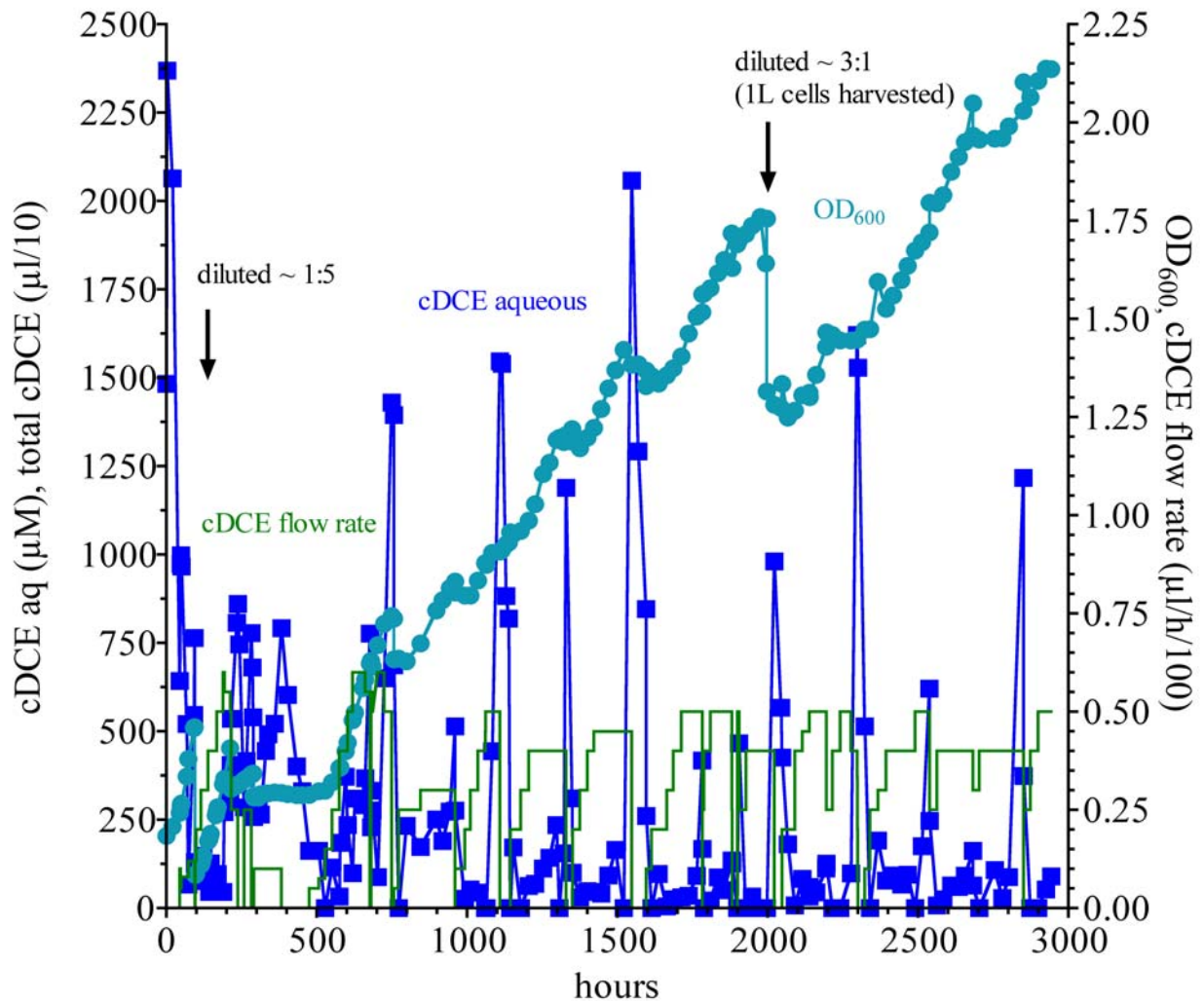
Figure 1.17 Growth of JS666 in 4-L Bioreactor.
