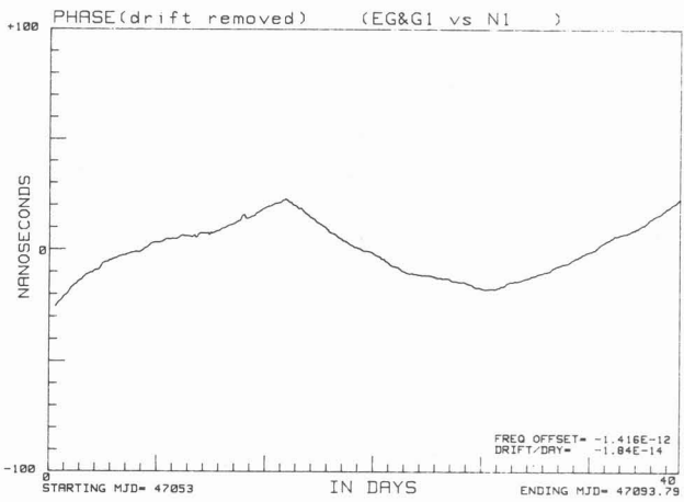
Figure 3. EG&G1 drift-corrected phase record.
