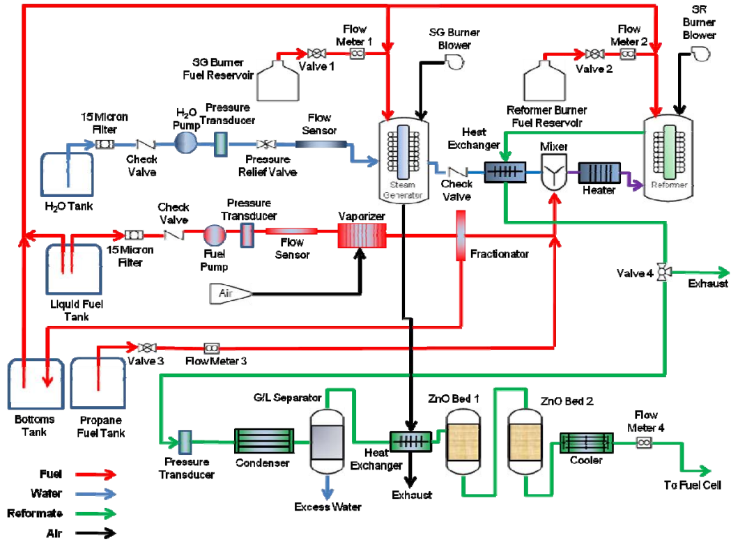
Figure A-1: Process's Flow Diagram
