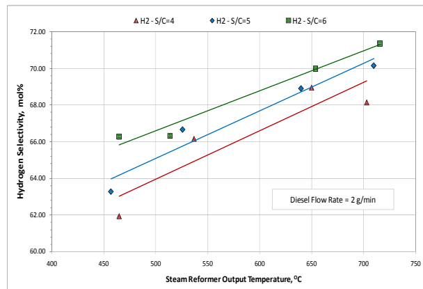
Figure 14: H 2 Selectivity as a Function of Diesel Reformate Temperature and S/C.
