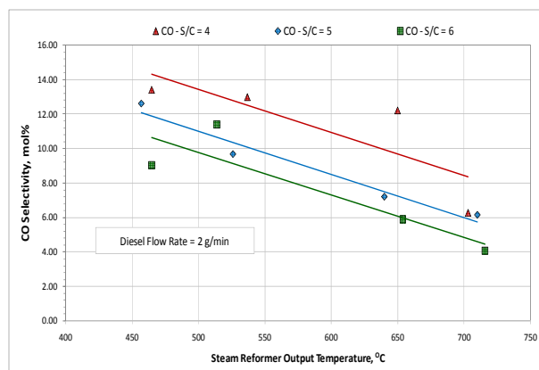
Figure 15: CO Selectivity as a Function of Diesel Reformate Temperature and S/C.
