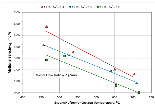
Figure 16: CH 4 Selectivity as a Function of Diesel Reformate Temperature and S/C.
