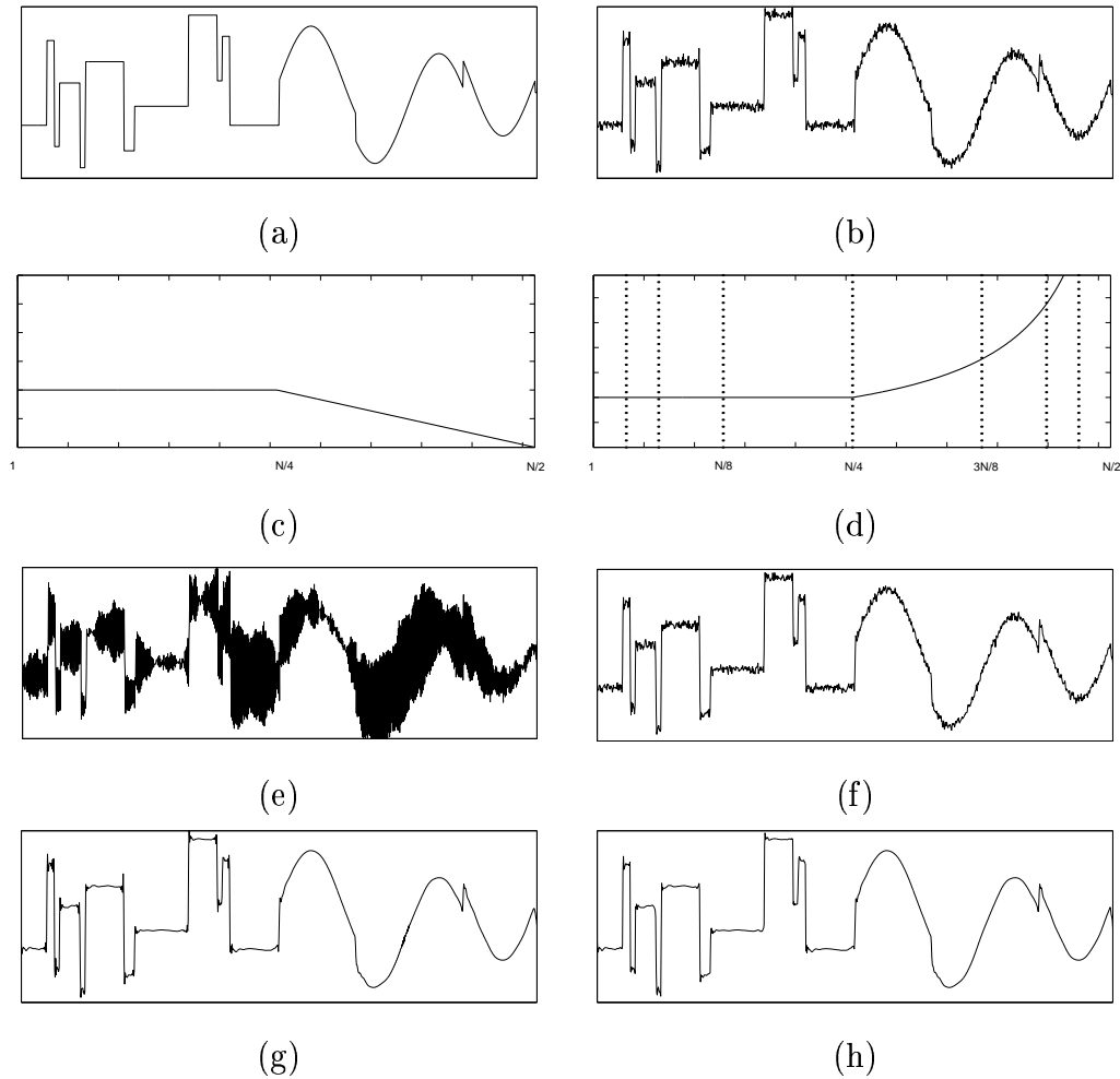
Figure 1.2 : (a) Test signal x ( N = 1024 ). It is a concatenation of Donoho's Blocks and Heavisine signals [5]. (b) Observed signal y ( MSE=0.0060 ). It is obtained by blurring x with by H and adding noise. (c) System frequency response H . It contains a zero at index \frac{N}{2} (index \frac{N}{2} corresponds to the normalized DFT frequency f = 0.5 ). (d) System Inverse frequency response H^{-1} . It amplifies noise at high frequencies. The mirror wavelet frequency splits for estimate (g) are shown with dashed vertical lines. (e) Pure inverse estimate ( MSE=1.1056 ). The pure inverse \frac{1}{H} amplifies all the high frequency noise components to give an extremely noisy estimate. (f) Wiener filter estimate ( MSE=0.0048 ). The Wiener filter is ineffective since the signal contains spatially localized phenomena such as edges; hence it provides an unsatisfactory estimate. (g) Mirror wavelet basis estimate [6, pp. 458–461] ( MSE=0.0027 ). The frequency splits (shown using dotted lines in (d)) aim to isolate the frequency where H goes to zero. The estimate performs better than the WVD method of [7] and conventional Wiener filter. (h) WaRD estimate with regularization \alpha^* = 0.06 , ( MSE=0.0017 ). The WaRD system tackles the noise amplification that stems from the action of H^{-1} (refer (d)) by employing partial Fourier-domain regularization followed by wavelet-domain estimation. It easily outperforms the mirror wavelet approach as well.
