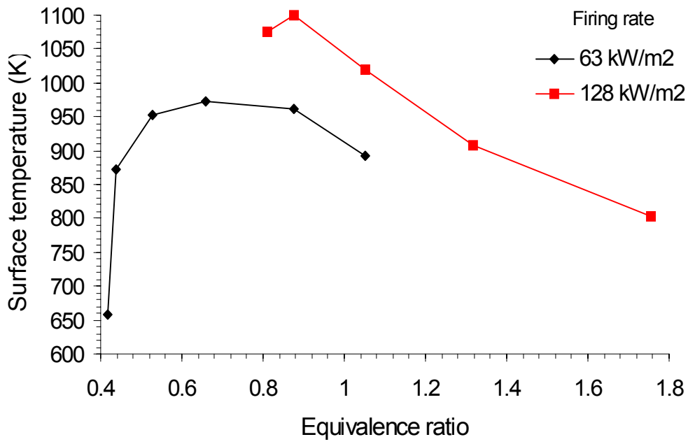
Figure 9 : Measured surface temperature of the porous burner for various equivalence ratios and for different firing rates( flatbed burner).
