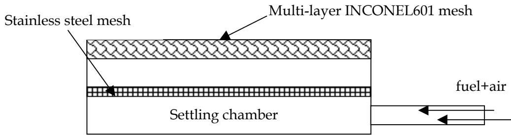
Figure 3: A schematic description of the components of the wire-mesh porous burner.
