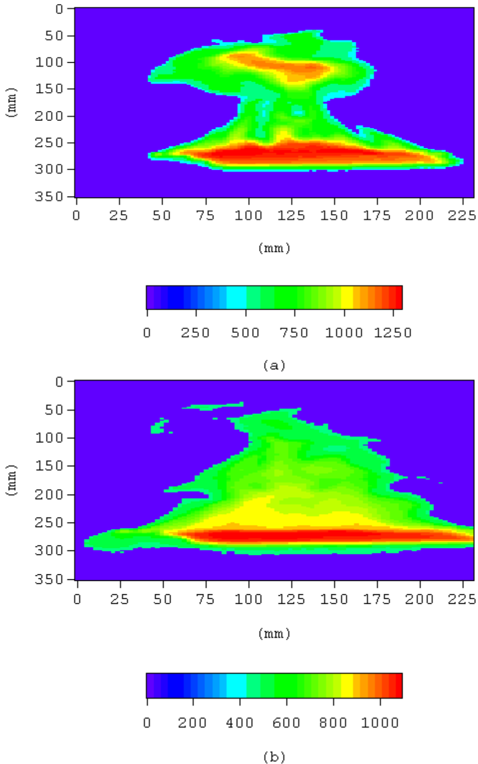
Figure 13: AGEMA's temperature contours ( ^{\circ}\text{C} ) from the flat-bed burner operating at a power density of (a) 63 \text{ kW/m}^2 , (b) 126 \text{ kW/m}^2 (a stoichiometric propane-air mixture).
