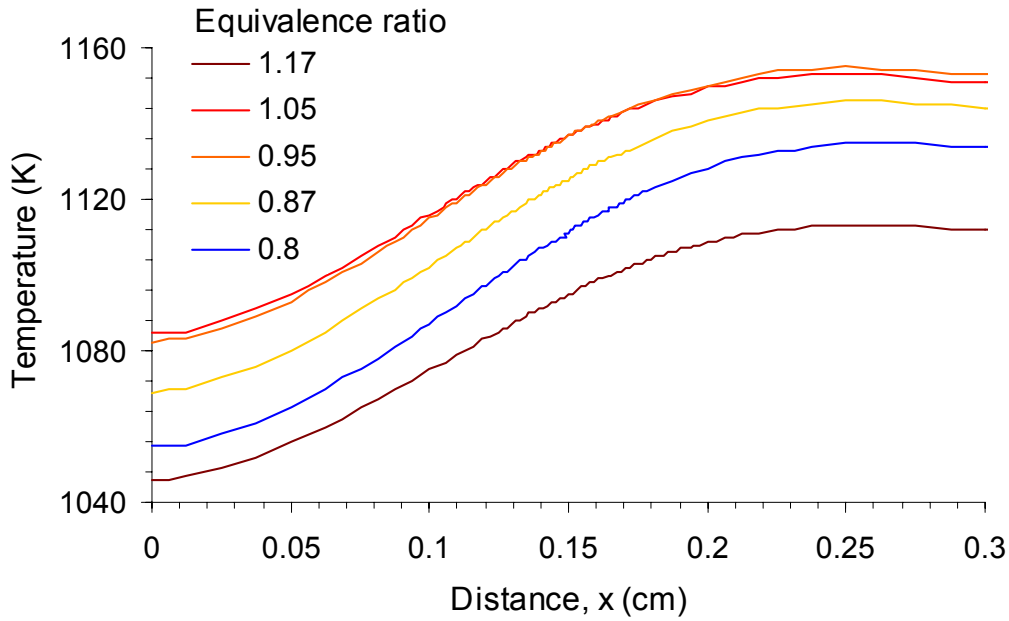
Figure 20: Computed distribution of solid temperature within the wire-mesh of the semi-cylindrical burner for various mixtures (power density of 417 \text{ kW/m}^2 ).
