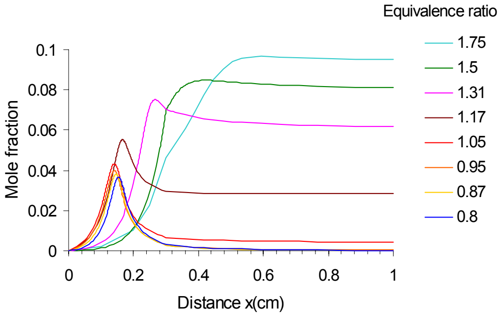
Figure 22: Carbon monoxide (CO) distribution for various mixtures.
