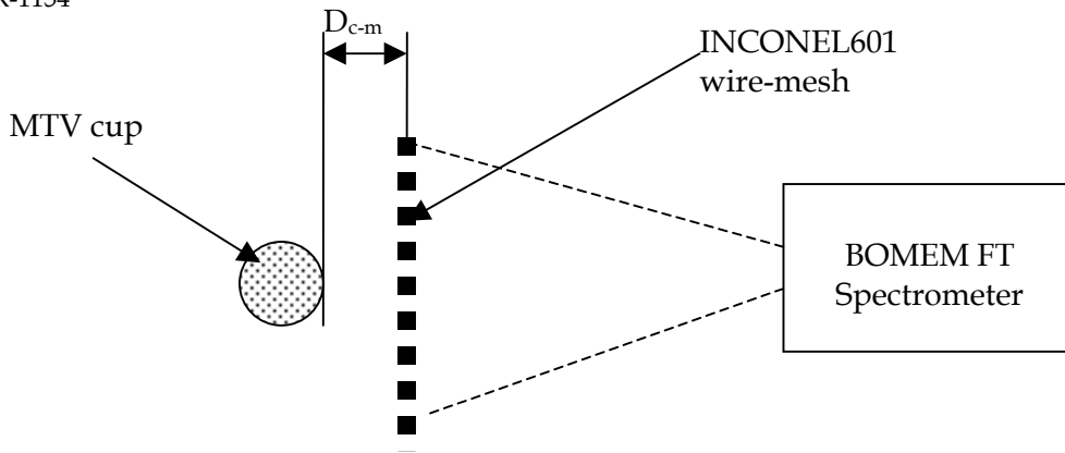
Figure 26: Layout of MTV-Wire-mesh experiment.
