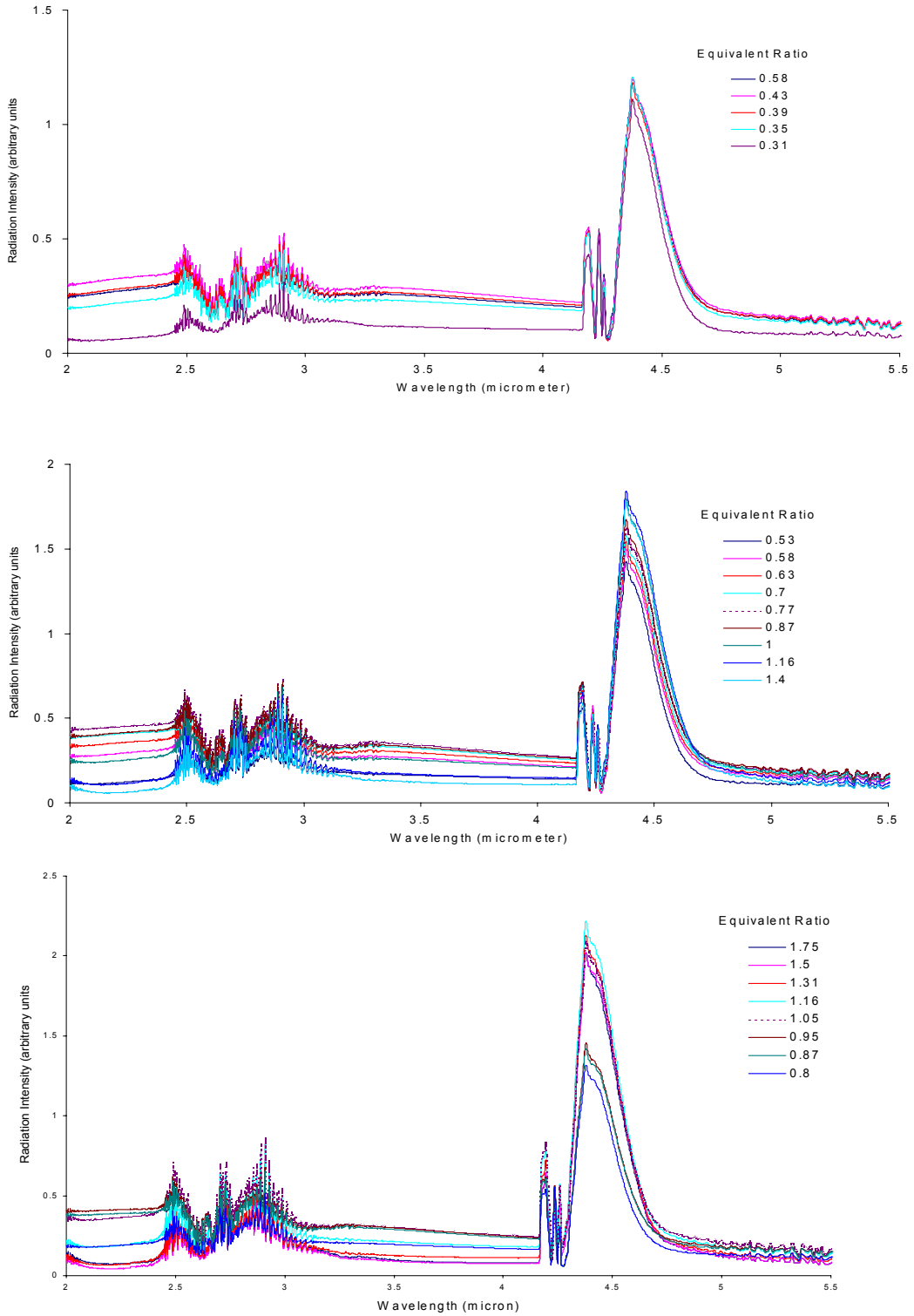
Figure 16: Spectral IR intensity over a waveband 2-5 \mu m, emitted from the semi-cylindrical burner operating at a power density of: (top) 139 kW/m 2 , (middle) 278 kW/m 2 , and (lower) 417 kW/m 2 , for various equivalence ratios
