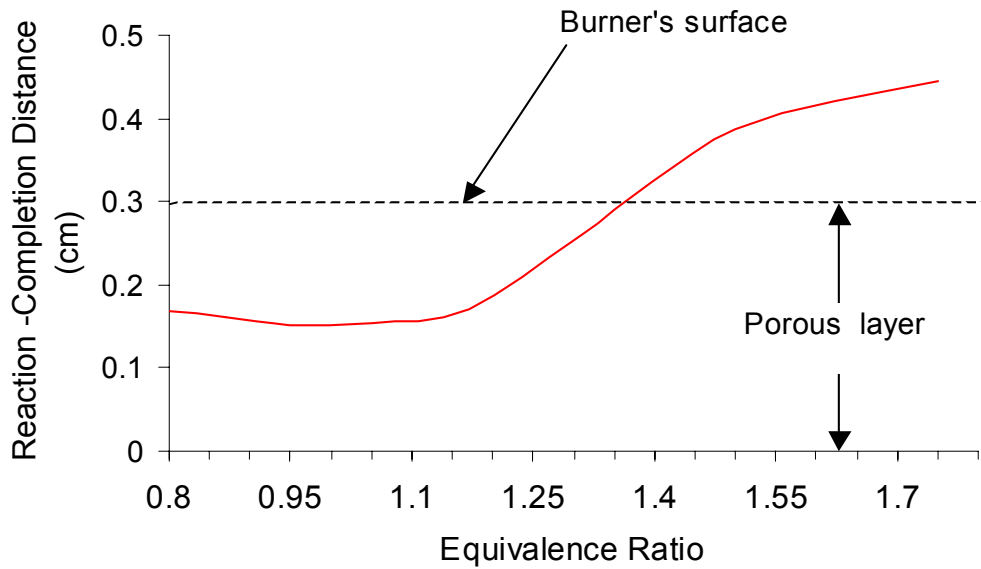
Figure 21: Effect of equivalence ratio on Reaction-Completion Distance.
