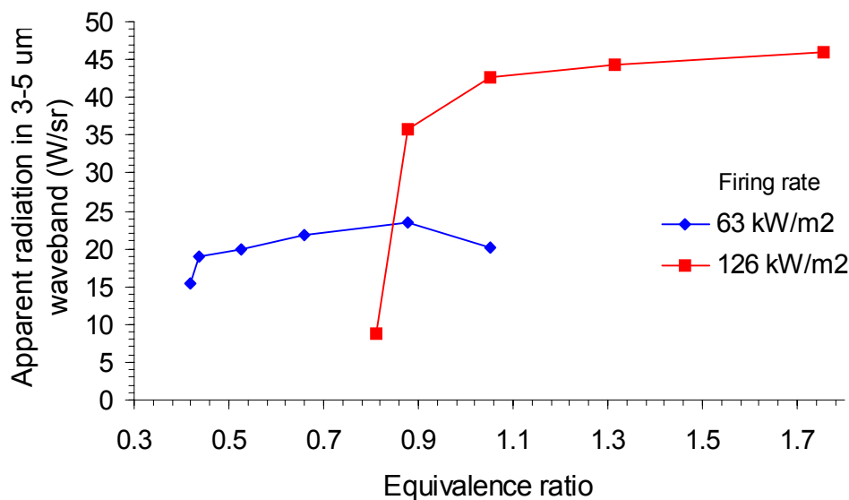
Figure 11: Apparent radiation in 3-5 micrometer waveband at various equivalence ratios and different firing rates (flat-bed burner).
