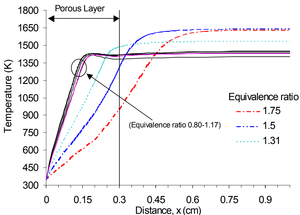
Figure 19: Computed gas temperature distribution of the semi-cylindrical burner for various equivalence ratios (power density of 417 \text{ kW/m}^2 ).
