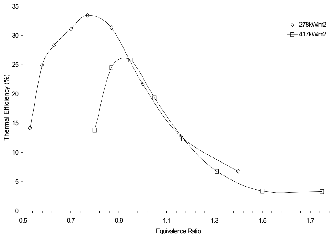
Figure 24: Measured thermal efficiency for various equivalence ratios.
