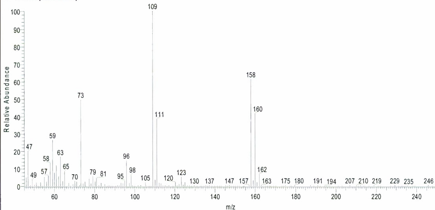
Figure 6. (a) Extracted ion GC-MS chromatogram for m/z 109 of HD standard solution (1ppm); (b) Electron impact mass spectrum of Yperite corresponding to the above chromatogram peak (full spectral scan).
