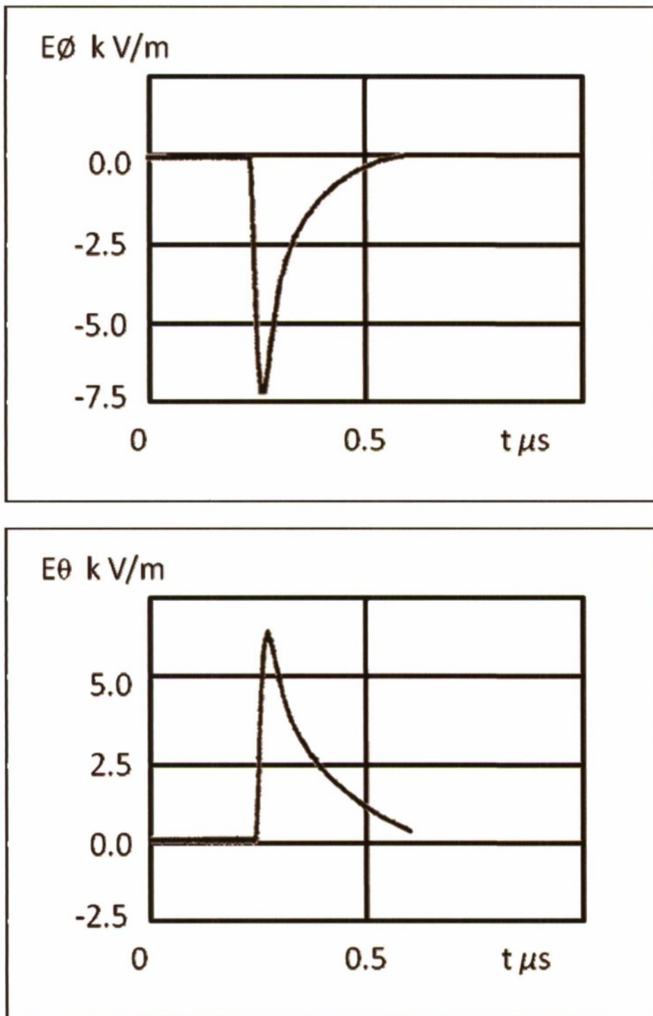
Figure 3. Computed Early-time HEMP Amplitudes from 1962 Kazakstan Event. 1
