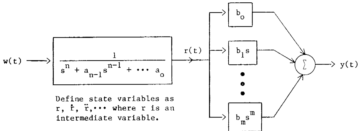
Figure 4 Shaping filter redrawn
