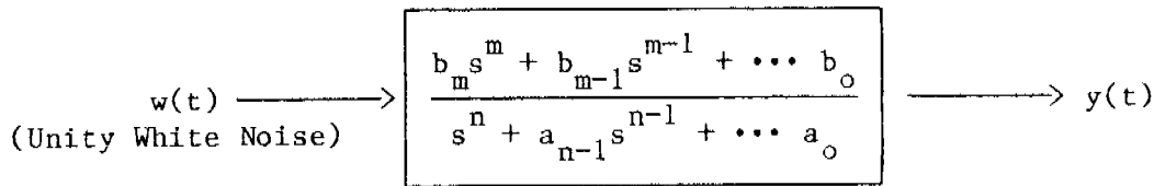
Figure 3 Shaping filter
