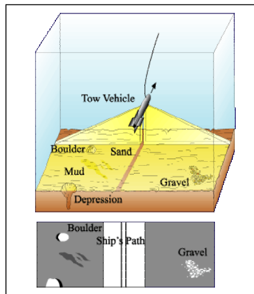
Figure 1. Towed SSS.
