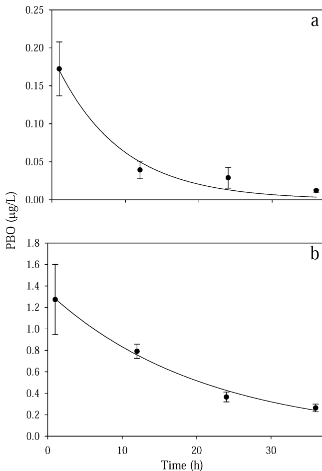
Fig. 2. Change in piperonyl butoxide (PBO) concentrations in water from 1 to 36 h after the spray with exponential decay curve for Princeton (a) (CA, USA; F = 21.37 , p = 0.0005 , r^2 = 0.622 , y = 0.5661e^{-1.2039x} ) and Colusa (b) (CA, USA; F = 11.53 , p = 0.004 , r^2 = 0.452 , y = 1.3446e^{-0.0478x} ).
