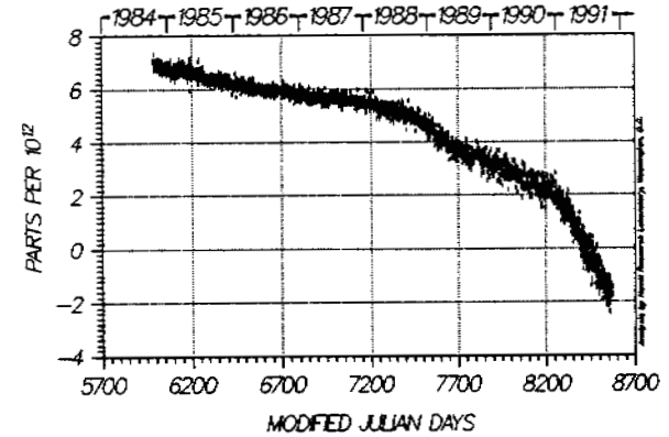
Figure 5. NAVSTAR 10 Frequency Offset.
