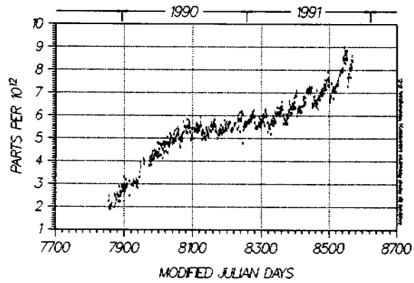
Figure 12. NAVSTAR 19 Frequency Offset.
