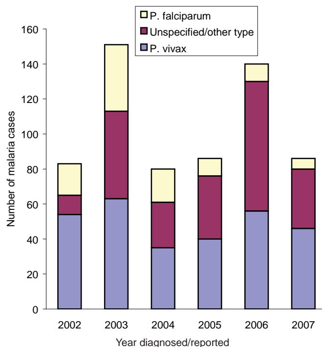
Figure 1. Malaria cases by plasmodium species and year, U.S. Armed Forces, 2002-2007
