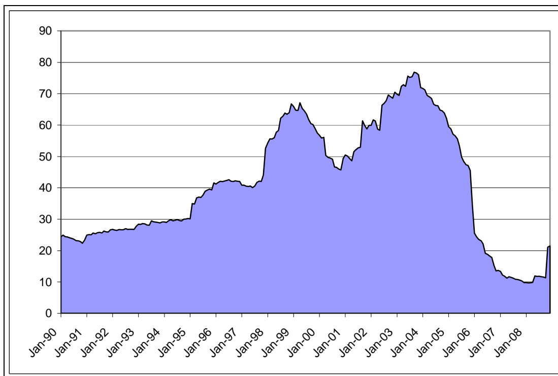
Figure I. Outstanding IMF Credit (1990-2008, SDR)
