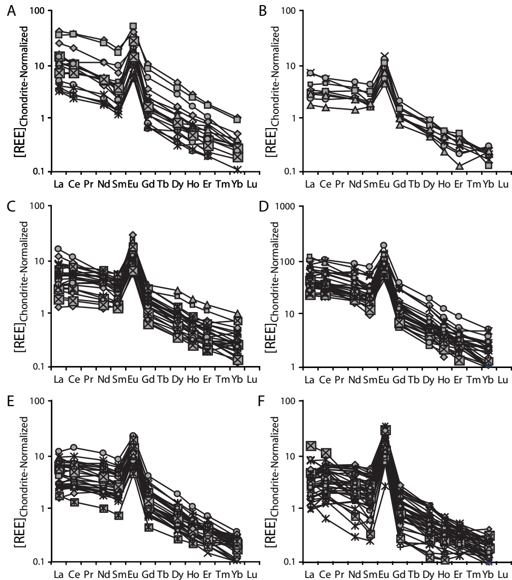
Figure 3.3. Chondrite-normalized REE patterns for massive anhydrite recovered from the seafloor at Fenway, PACMANUS hydrothermal system. Individual patterns determined in situ by laser ablation ICP-MS. A) sample J2_210_8_R2, B) sample J2_212_7_R1, C) sample J2_216_1_R1, D) sample J2_216_5_R1, E) sample J2_216_12_R1, F) sample J2_216_14_R1. Chondritic values from Anders and Grevasse (1989).
