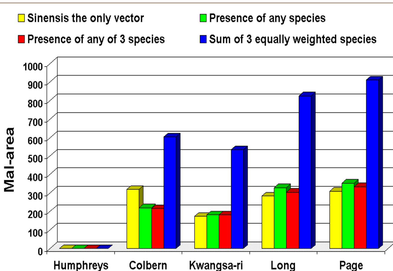
Figure 6. Mal-area calculations in number of one-km 2 pixels for malaria within 10 km of 5 US military installations in the ROK, based on vector distribution models and the areas predicted suitable for malaria, from the Malaria Atlas Project.
