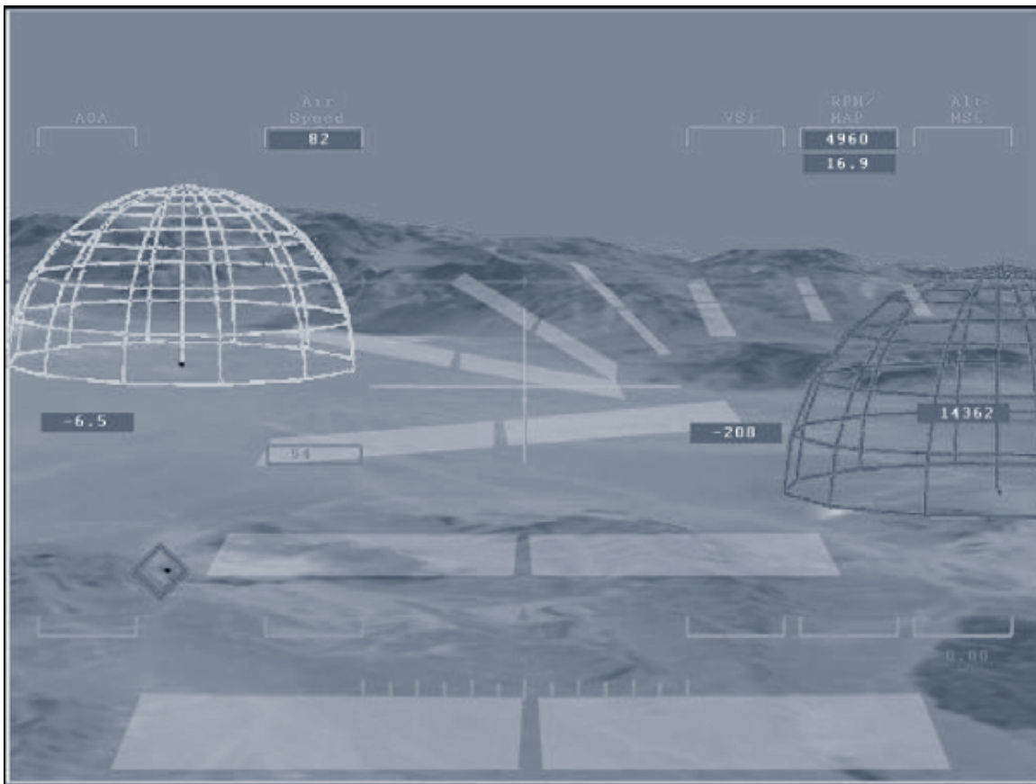
Figure 6. Synthetic threat and pathway information overlaid on a simulated nose camera imagery. From Calhoun et al., 2005. Reprinted with permission.
