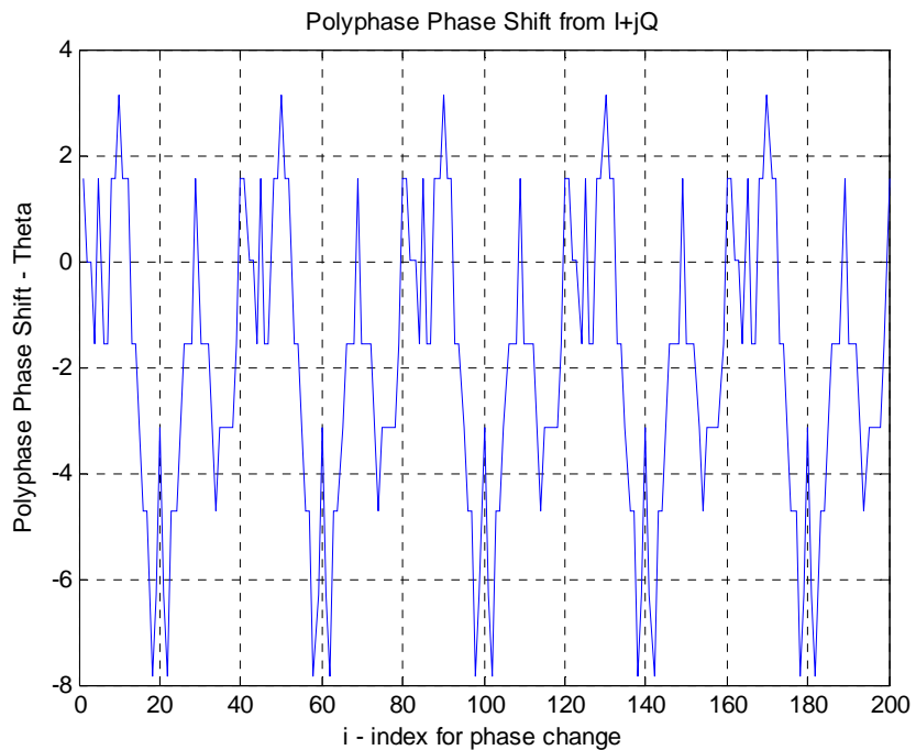
Figure 3. OPS Sequence with N_c = 40 , L = 4 , M = 4 Code Set 1 showing five periods of phase shifts (degrees).
