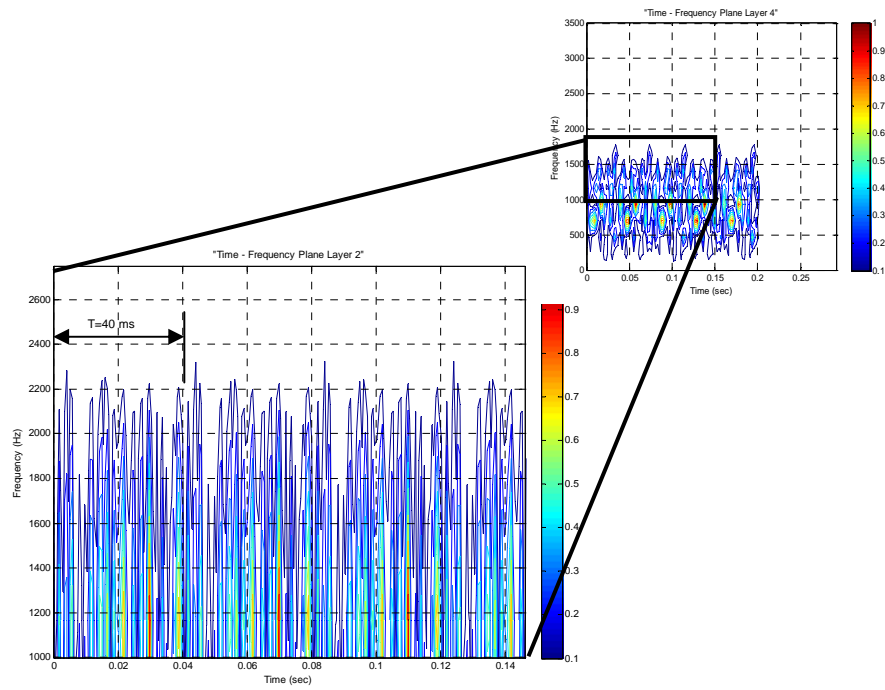
Figure 71. QMFB Layer 2 of Optimized OPS 40 Code 1 code period T = 40 ms.
