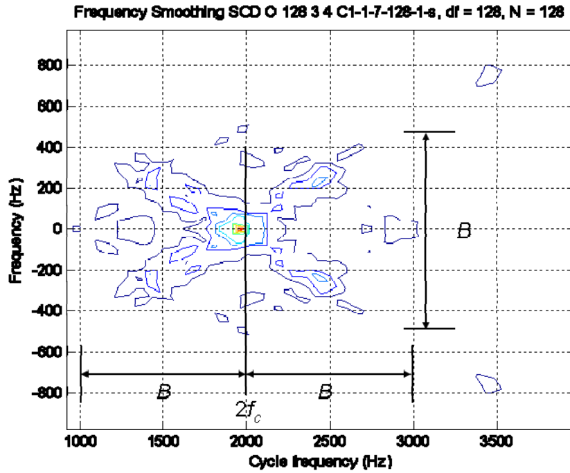
Figure 79. DFMS of OPS 128 Code 1 with T = 128 ms and B = 1000 Hz Individual Modulation Quadrant.
