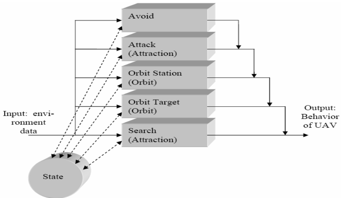
Figure 90. UAV Control Structure in Java Program.
