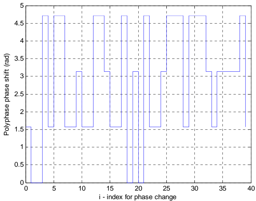
Figure 2. OPS Sequence with N_c = 40 , L = 4 , M = 4 Code Set 1 showing one period of phase shifts (radians).
