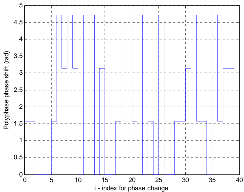
Figure 11. OPS Sequence with N_c = 40 , L = 4 , M = 4 Code Set 4 showing one period of phase shifts (radians).
