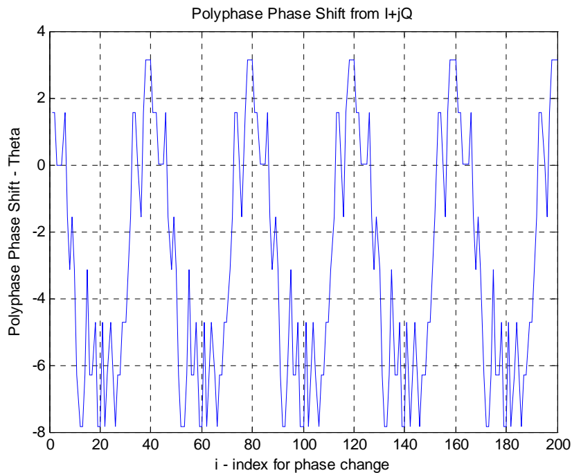
Figure 12. OPS Sequence with N_c = 40 , L = 4 , M = 4 Code Set 4 showing five periods of phase shifts (degrees).
