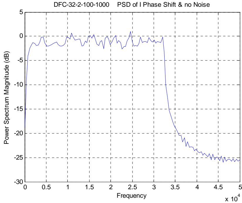
Figure 51. Power Spectral Density of DFC Set 2 (Signal Only).
