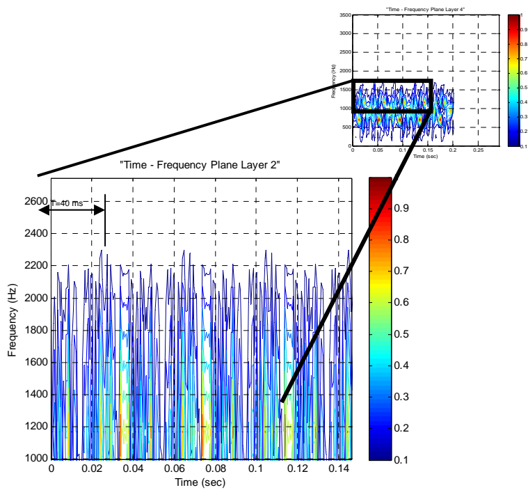
Figure 67. QMFB Layer 2 of OPS 40 Code 1 with code period T = 40 \text{ ms} .
