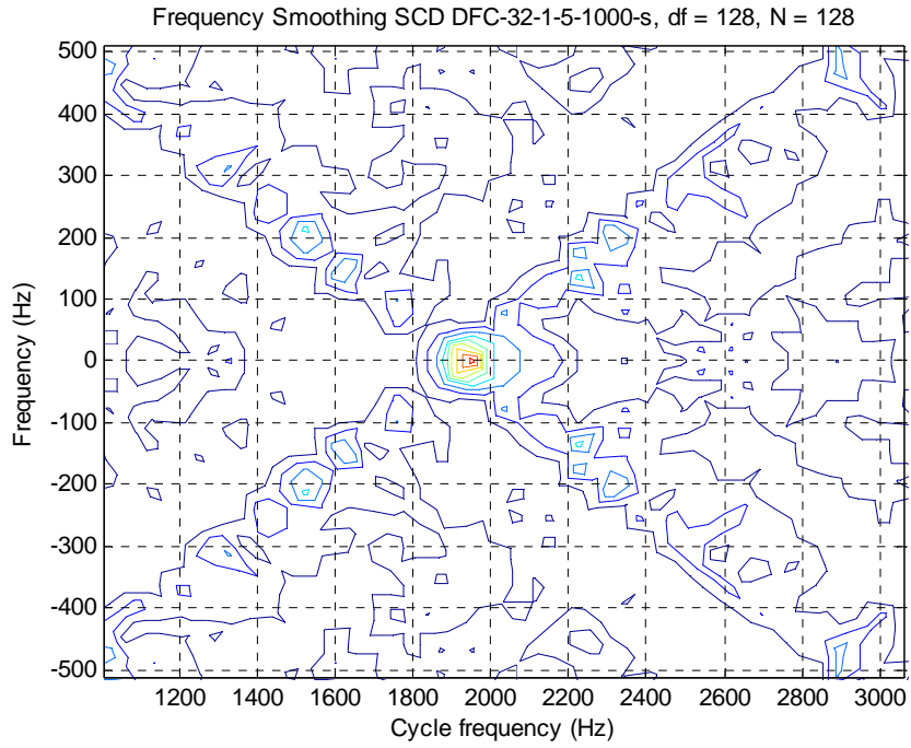
Figure 87. DFMS of DFC 32 Code 1 with f = 1000 Hz Individual Modulation Quadrant.
