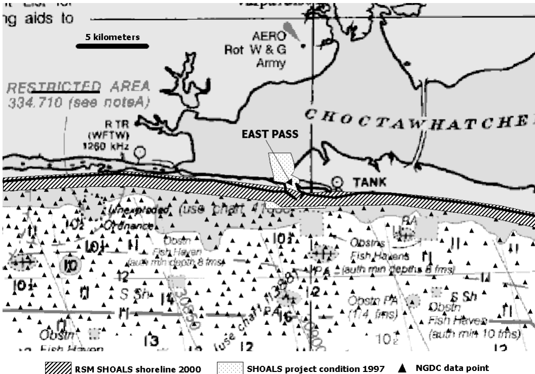
Figure 5. East Pass, Florida. Graphical representation of data retained for RSM baseline data set. Triangles represent actual NGDC data points while SHOALS 4- to 8-meter density data sets are represented by filled polygons.
