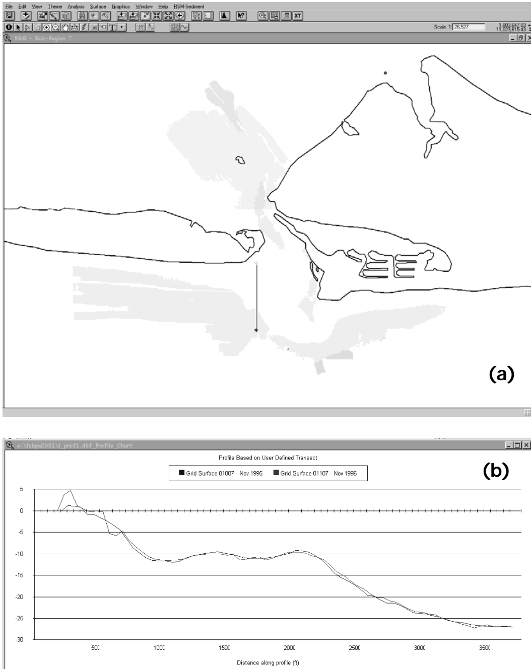
Figure 9. Profile tool created for RSM GIS. Figure 9a shows the spatial domain of the RSM GIS near East Pass, Florida. This view includes the shoreline in this area, the grid created for the 1996 SHOALS data set, and a line where a profile is desired. Figure 9b shows the profile viewing window, where a profile is displayed for the November 1995 SHOALS survey and the 1996 SHOALS survey.
