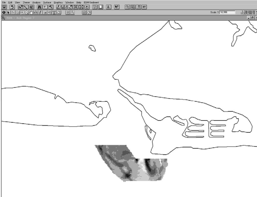
Figure 10. Volume tool created for RSM GIS. This figure shows the spatial domain for the RSM GIS near East Pass, Florida. The view includes the shoreline and the difference grid computed during a volume calculation. The black and dark gray grid cells are areas of positive difference, or accretion. The lighter gray grid cells are areas of negative difference, or erosion.
