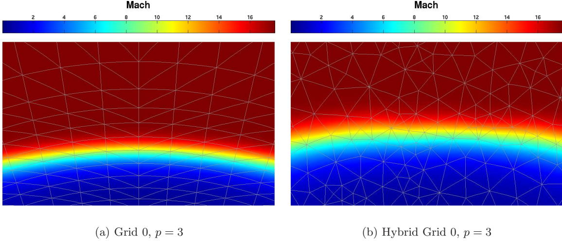
Figure 6-21: Mach contours at the bow shock of flow over 2D half cylinder with M_\infty = 17.605 , \text{Re} = 376,930 ( p = 3 solution).
