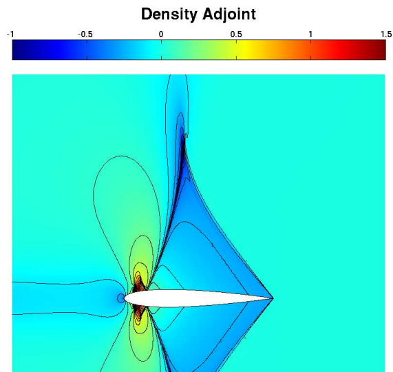
(c) Near-field
