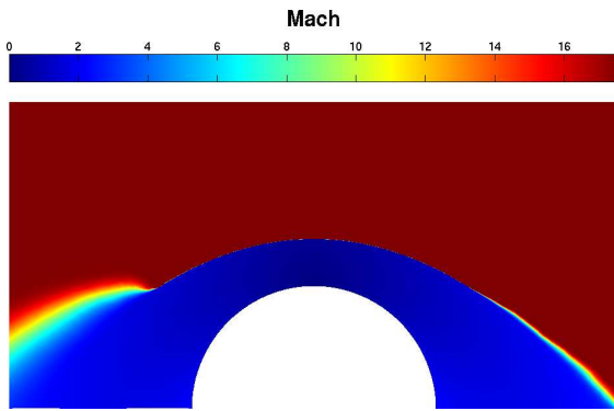
(c) Mach
