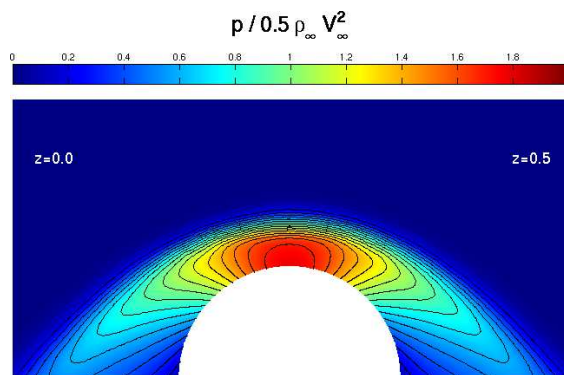
(c) Pressure
