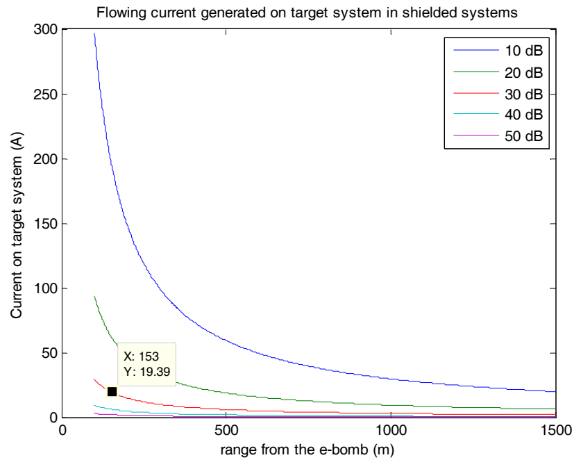
Figure 29. Current vs. the range plot of moderate e-bomb for shielded systems
