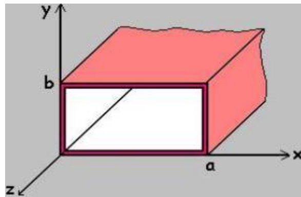
Figure 17. Waveguide dimensions
