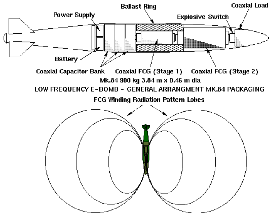
FIG.4 LOW FREQUENCY E-BOMB WARHEAD (MK.84 FORM FACTOR)
