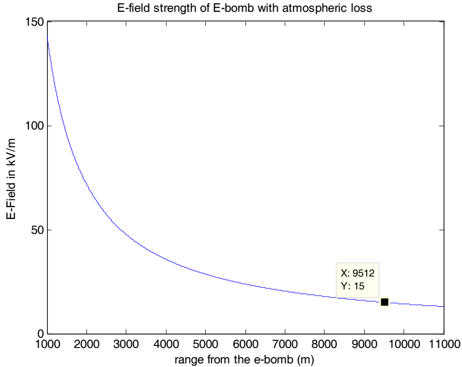
Figure 51. High-tech e-bomb potential lethality range for Swedish Fighter Aircraft
