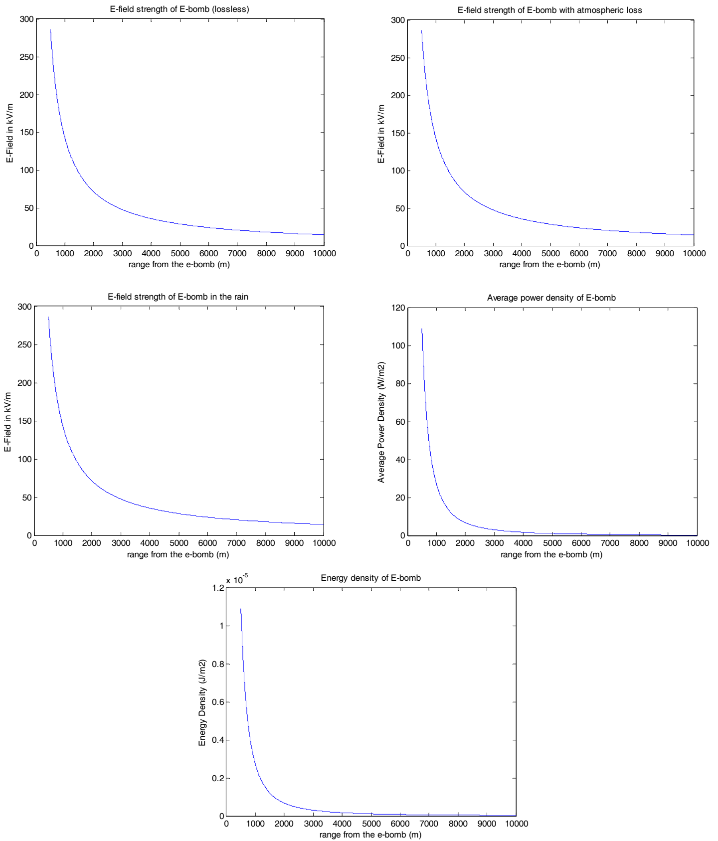
Figure 46. Simulation output for high-tech e-bomb 89
