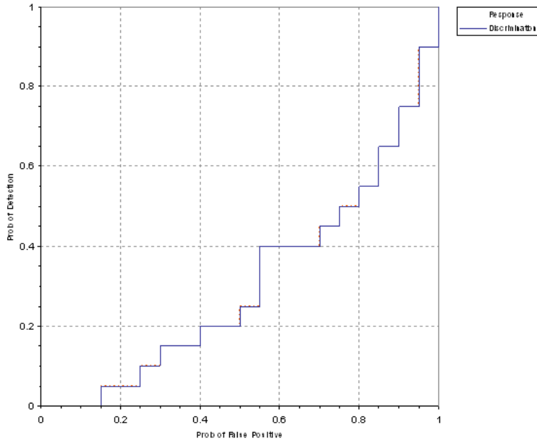
Figure 4. MAG G823/sling blind grid probability of detection for response and discrimination stages versus their respective probability of false positive for all ordnance larger than 20 mm.
