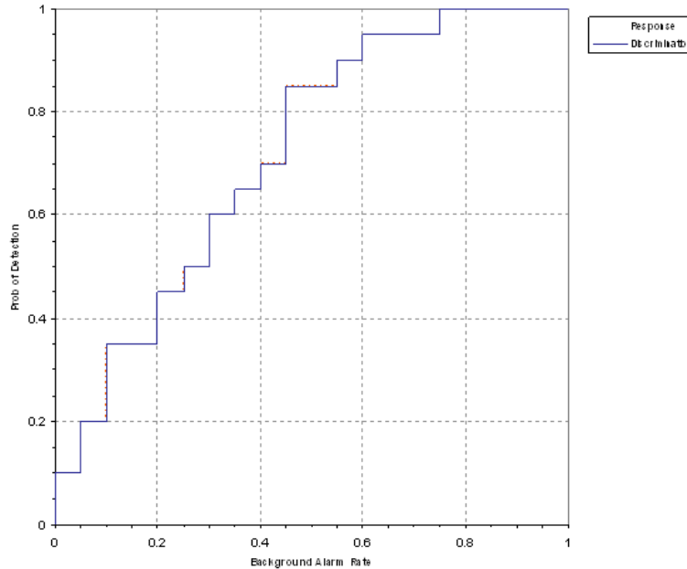
Figure 3. MAG G823/sling blind grid probability of detection for response and discrimination stages versus their respective background alarm rate over all ordnance categories combined.
