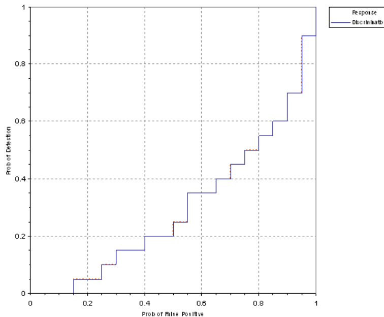
Figure 2. MAG G823/sling blind grid probability of detection for response and discrimination stages versus their respective probability of false positive over all ordnance categories combined.
