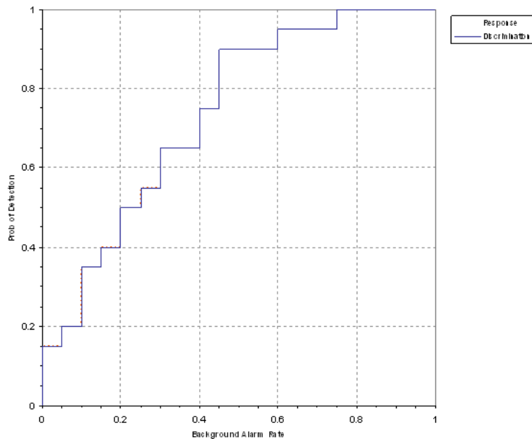
Figure 5. MAG G823/sling blind grid probability of detection for response and discrimination stages versus their respective background alarm rate for all ordnance larger than 20 mm.
