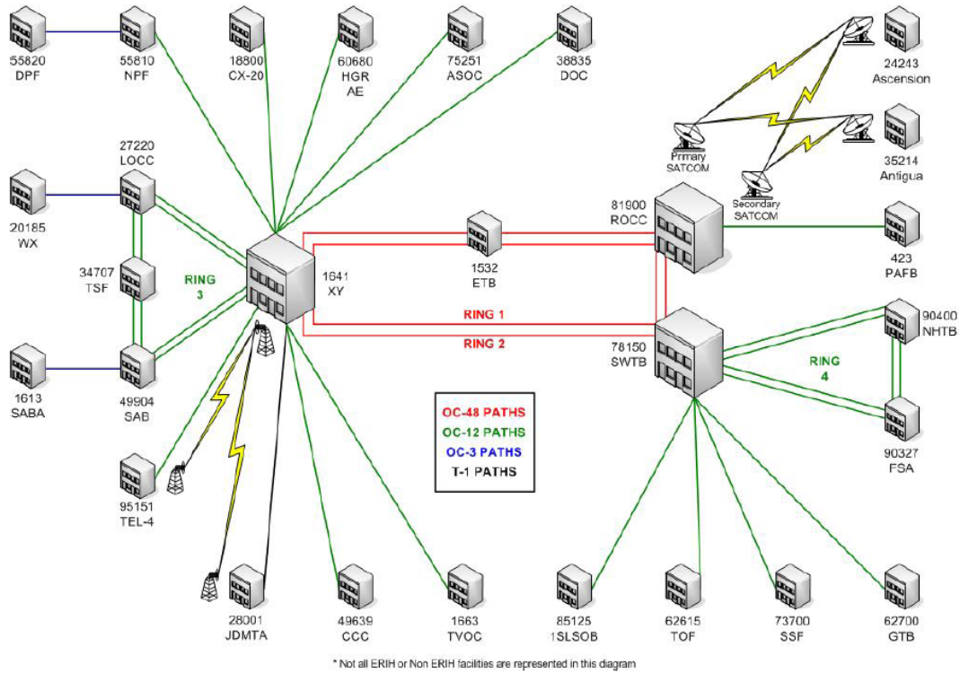
Figure 3. Eastern Range Core Network (Fig. 1-1 in Computer Sciences Raytheon, 2008 )
