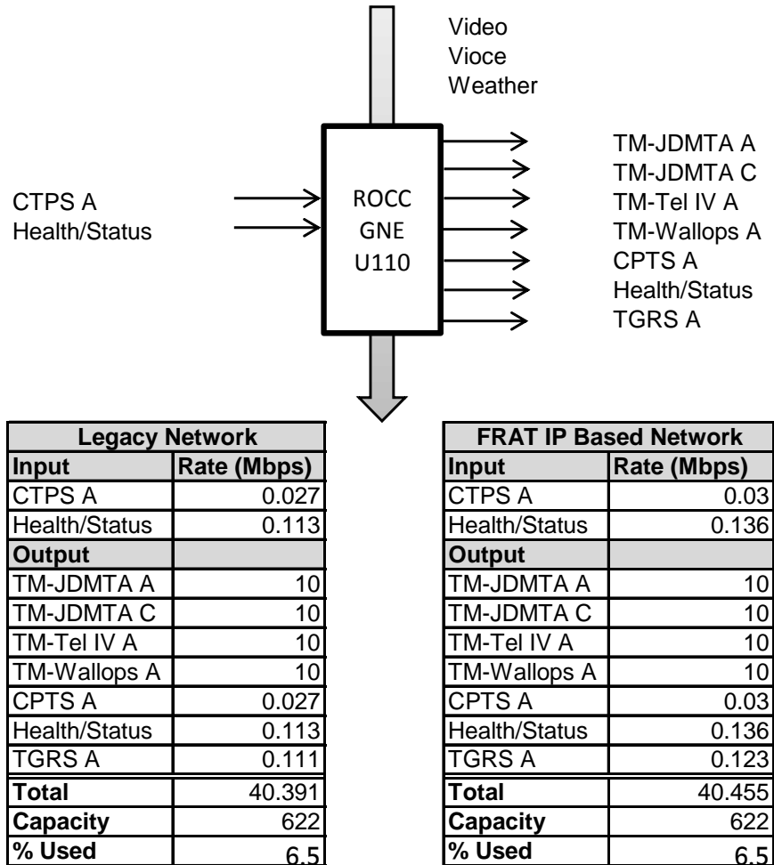
Figure 15. Core Node Connected to CTPS
