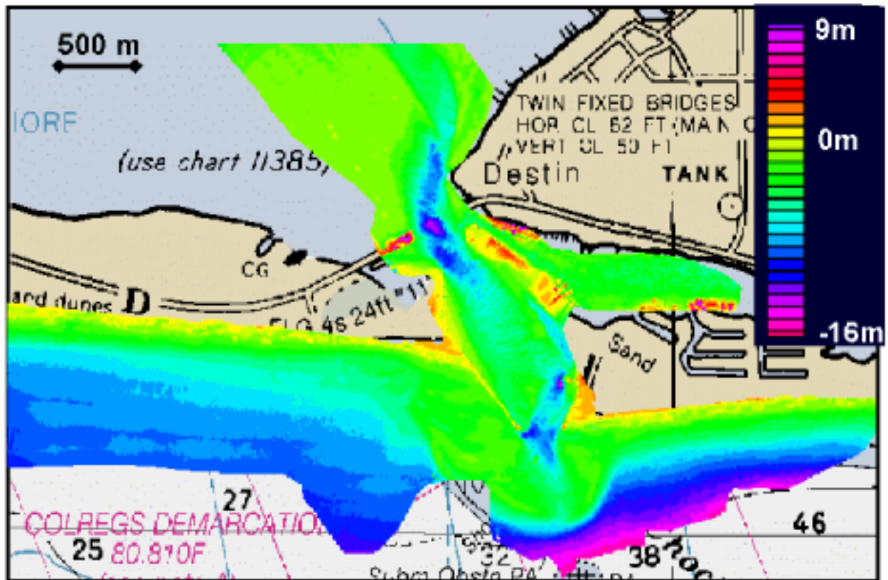
Figure 9. East Pass, Florida, U.S.A. NOAA nautical chart with contours of SHOALS data, December 1996.
