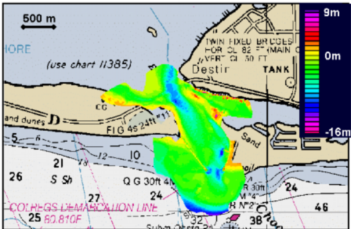
Figure 8. East Pass, Florida, U.S.A. NOAA nautical chart with contours of SHOALS data, October 1995.
