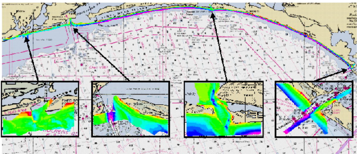
Figure 2. RSM DP terrain model generated with SHOALS data.
