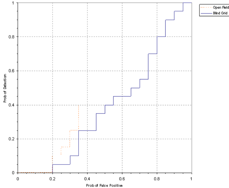
Figure 9. MAG G823/sling P_d^{disc} versus the respective P_{fp} for ordnance larger than 20 mm.
