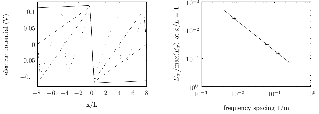
Figure A.1: (left) The electric potential \Phi at z = -H'/H for multiple values of m . The dotted line is for m = 4 , the dashed-dotted for m = 8 , the dashed for m = 16 , and the solid for m = 256 . Note the a non-zero slope outside of the jet ( |x/L| < 1/2 ) that corresponds to a non-zero horizontal electric field, and that for lower values of m the domain is small enough to show that the solution is periodic with period mx/L . The solution is under-resolved in x for |x/L| > 1 . The offset of \bar{E}_x / \max(\bar{E}_x) plotted against the frequency resolution 1/M (right). The slope of the best-fit line is -1.028 \pm 0.007 . The parameters used are: H = 3000 , H' = 500 , H_s = 6000 m, L = 100 km, and \sigma_s/\sigma = 0.4 .
