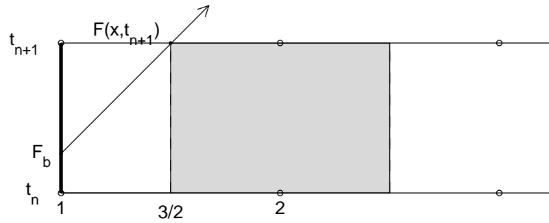
Fig. 3. Same as Fig. 2 except at the left boundary of the integration domain.
