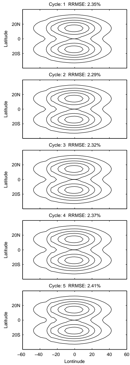
Fig. 7. Surface elevation \phi(s, y, t) of the Rossby soliton after 1-5 cycles around the earth obtained from numerical integration with C = 1.5 using the TFSL scheme.
