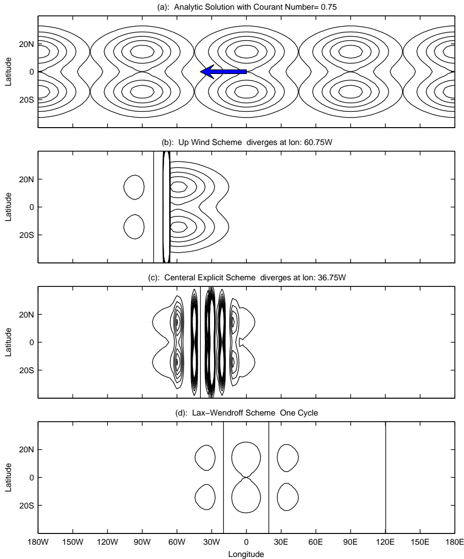
Fig. 1. Surface elevation \phi(s, y, t) of the Rossby solitons obtained from (a) exact solution, and numerical integration with C = 0.75 using (b) upwind scheme, (c) central scheme, and (d) Lax-Wendroff scheme. Note that the numerical solution diverges at 60^{\circ}45'W using the upwind scheme and 38^{\circ}45'W using the central scheme. The numerical solution does not diverge using the Lax-Wendroff scheme, however, the solution is totally distorted from the analytical solution after propagating one cycle around the earth.
