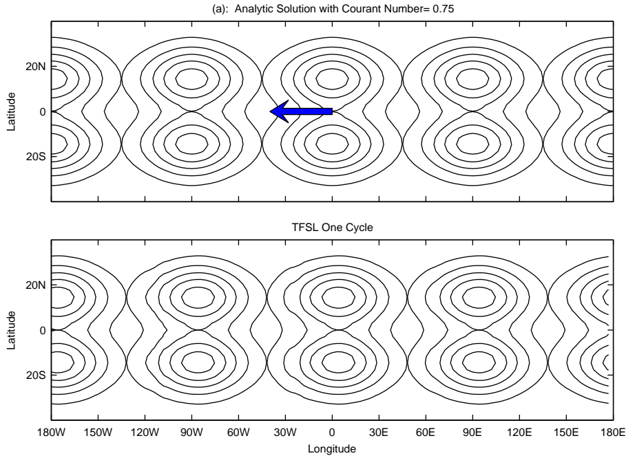
Fig. 6. Surface elevation \phi(s, y, t) of the Rossby soliton obtained from (a) exact solution, and numerical integration with C = 0.75 using (b) TFSL-scheme. The solutions \phi(s, y, t) are plotted at four time instances for the Rossby soliton (exact solution) westward propagating 90^\circ , 180^\circ , 270^\circ , and 360^\circ (return to the initial location).
