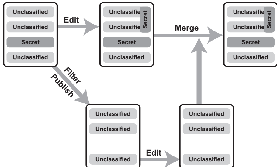
Figure 2: DocServer Merge Operations
