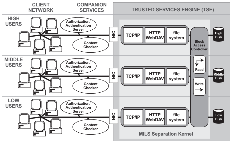
Figure 1: Trusted Services Engine (TSE) Architecture
